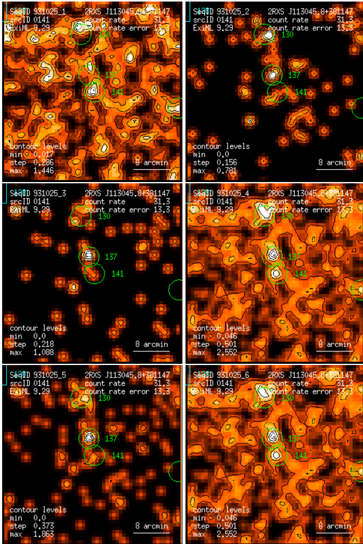
Figure 141: RASS 931025: detection 0141: band rate images, Gaussian filter: (1) PSPC channels 11 – 41, (2) 52 – 90, (3) 91 – 201, (4) 11 – 235, (5) 52 – 201, (6) 11 – 201. Broad band rates in counts/ks. Band rate contour levels in counts/ks/arcmin 2 .
