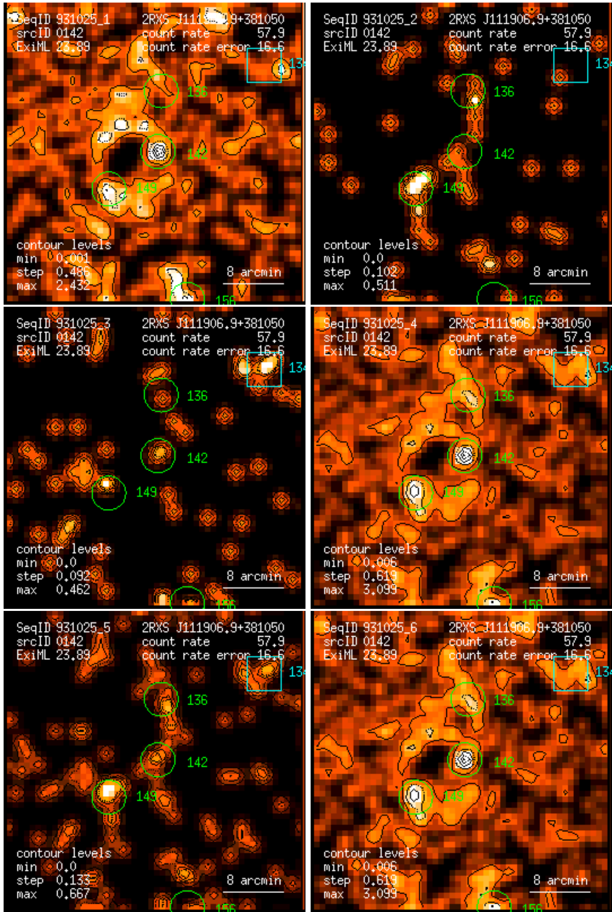
Figure 142: RASS 931025: detection 0142: band rate images, Gaussian filter: (1) PSPC channels 11 – 41, (2) 52 – 90, (3) 91 – 201, (4) 11 – 235, (5) 52 – 201, (6) 11 – 201. Broad band rates in counts/ks. Band rate contour levels in counts/ks/arcmin 2 .
