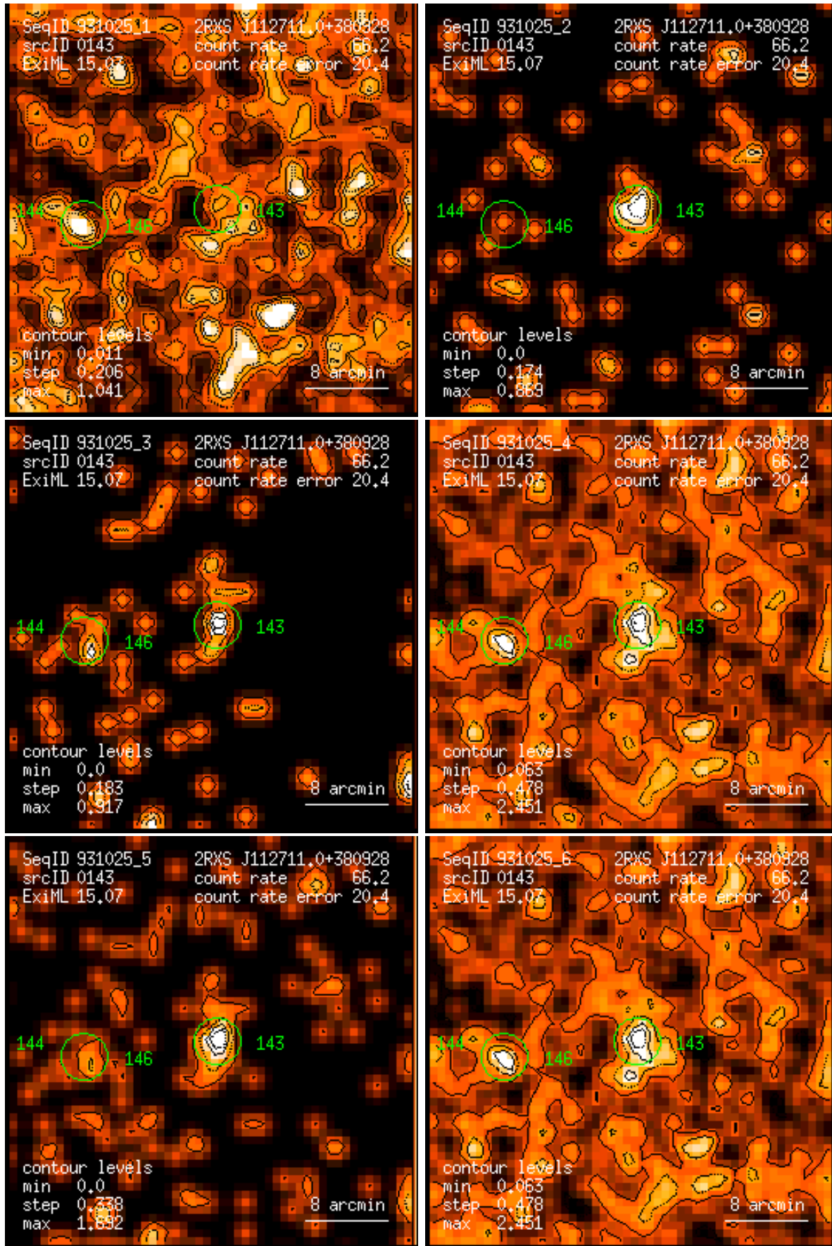
Figure 143: RASS 931025: detection 0143: band rate images, Gaussian filter: (1) PSPC channels 11 – 41, (2) 52 – 90, (3) 91 – 201, (4) 11 – 235, (5) 52 – 201, (6) 11 – 201. Broad band rates in counts/ks. Band rate contour levels in counts/ks/arcmin 2 .
