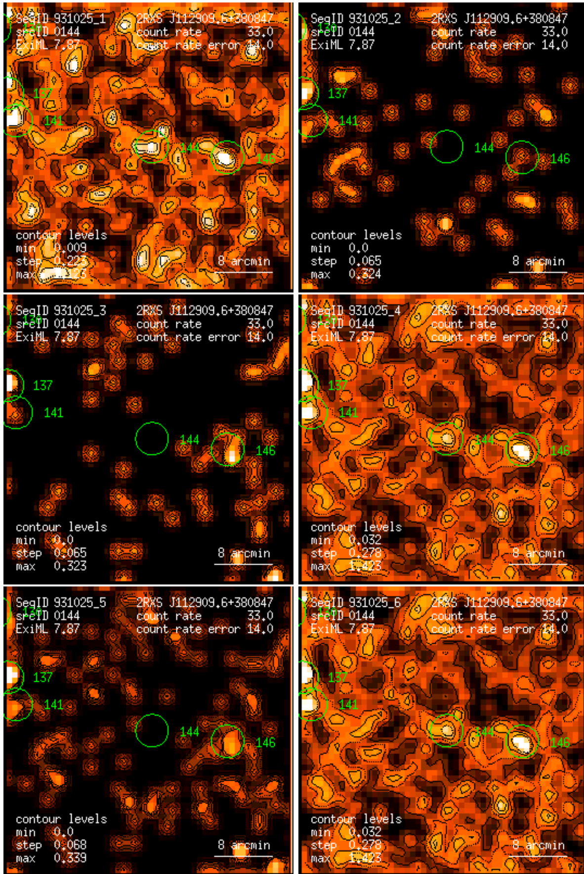
Figure 144: RASS 931025: detection 0144: band rate images, Gaussian filter: (1) PSPC channels 11 – 41, (2) 52 – 90, (3) 91 – 201, (4) 11 – 235, (5) 52 – 201, (6) 11 – 201. Broad band rates in counts/ks. Band rate contour levels in counts/ks/arcmin 2 .
