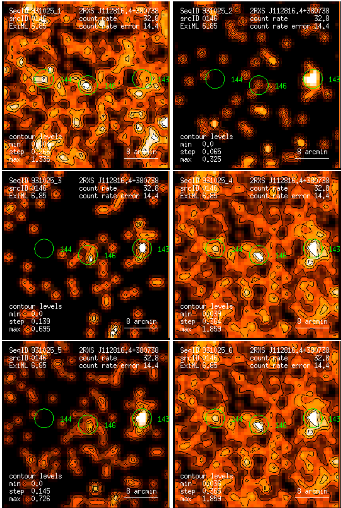
Figure 146: RASS 931025: detection 0146: band rate images, Gaussian filter: (1) PSPC channels 11 – 41, (2) 52 – 90, (3) 91 – 201, (4) 11 – 235, (5) 52 – 201, (6) 11 – 201. Broad band rates in counts/ks. Band rate contour levels in counts/ks/arcmin 2 .
