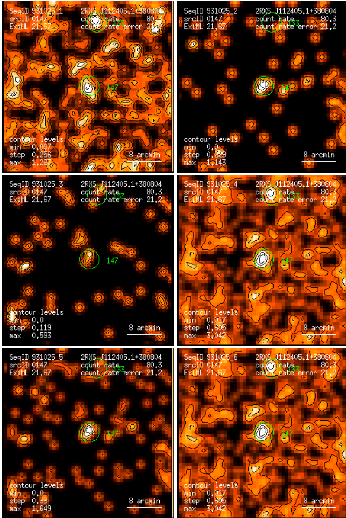
Figure 147: RASS 931025: detection 0147: band rate images, Gaussian filter: (1) PSPC channels 11 – 41, (2) 52 – 90, (3) 91 – 201, (4) 11 – 235, (5) 52 – 201, (6) 11 – 201. Broad band rates in counts/ks. Band rate contour levels in counts/ks/arcmin 2 .
