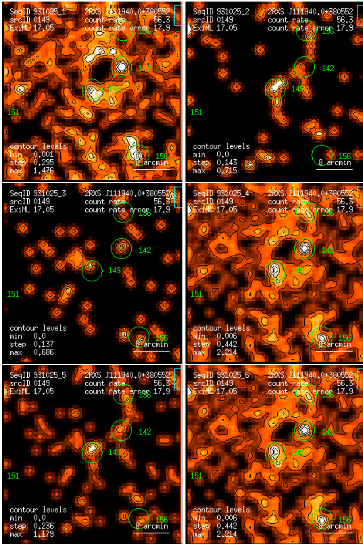
Figure 149: RASS 931025: detection 0149: band rate images, Gaussian filter: (1) PSPPC channels 11 – 41, (2) 52 – 90, (3) 91 – 201, (4) 11 – 235, (5) 52 – 201, (6) 11 – 201. Broad band rates in counts/ks. Band rate contour levels in counts/ks/arcmin 2 .
