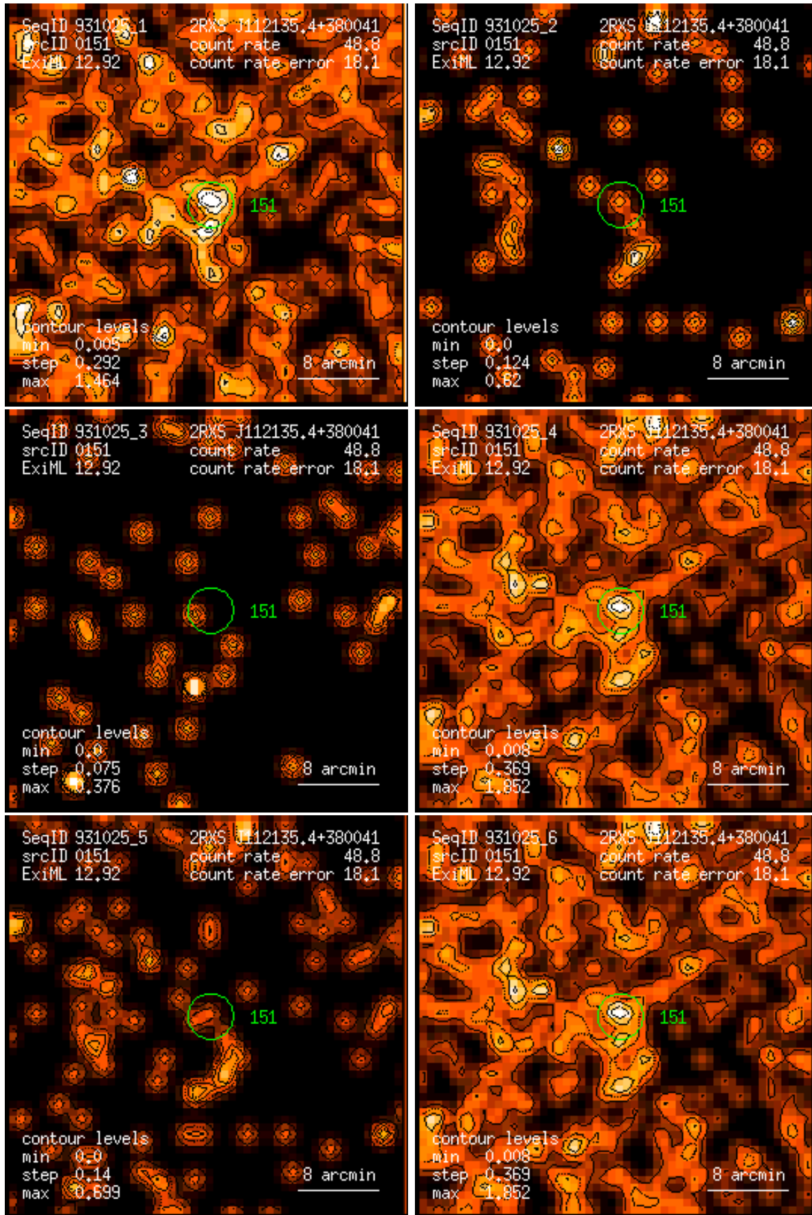
Figure 151: RASS 931025: detection 0151: band rate images, Gaussian filter: (1) PSPC channels 11 – 41, (2) 52 – 90, (3) 91 – 201, (4) 11 – 235, (5) 52 – 201, (6) 11 – 201. Broad band rates in counts/ks. Band rate contour levels in counts/ks/arcmin 2 .
