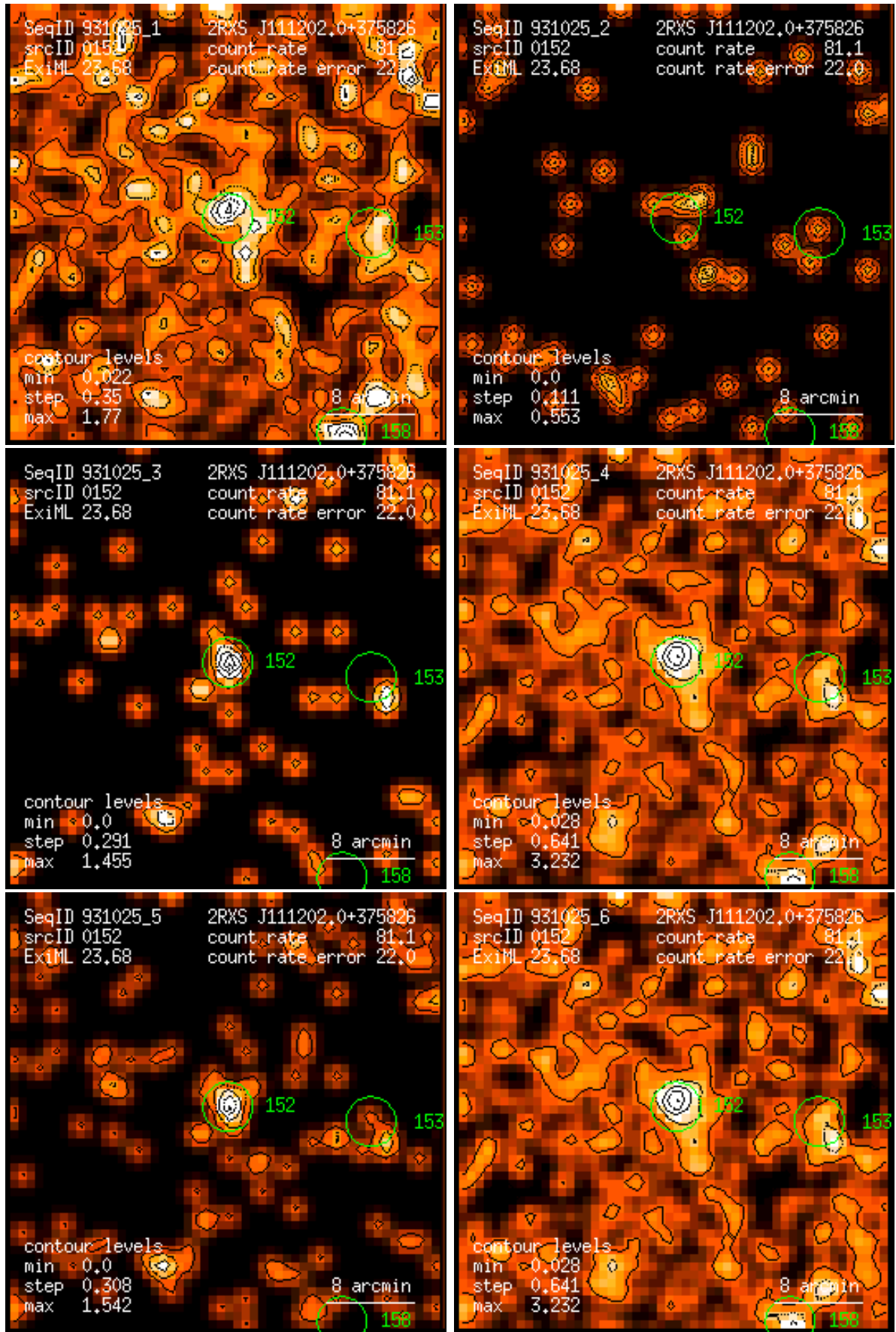
Figure 152: RASS 931025: detection 0152: band rate images, Gaussian filter: (1) PSPC channels 11 – 41, (2) 52 – 90, (3) 91 – 201, (4) 11 – 235, (5) 52 – 201, (6) 11 – 201. Broad band rates in counts/ks. Band rate contour levels in counts/ks/arcmin 2 .
