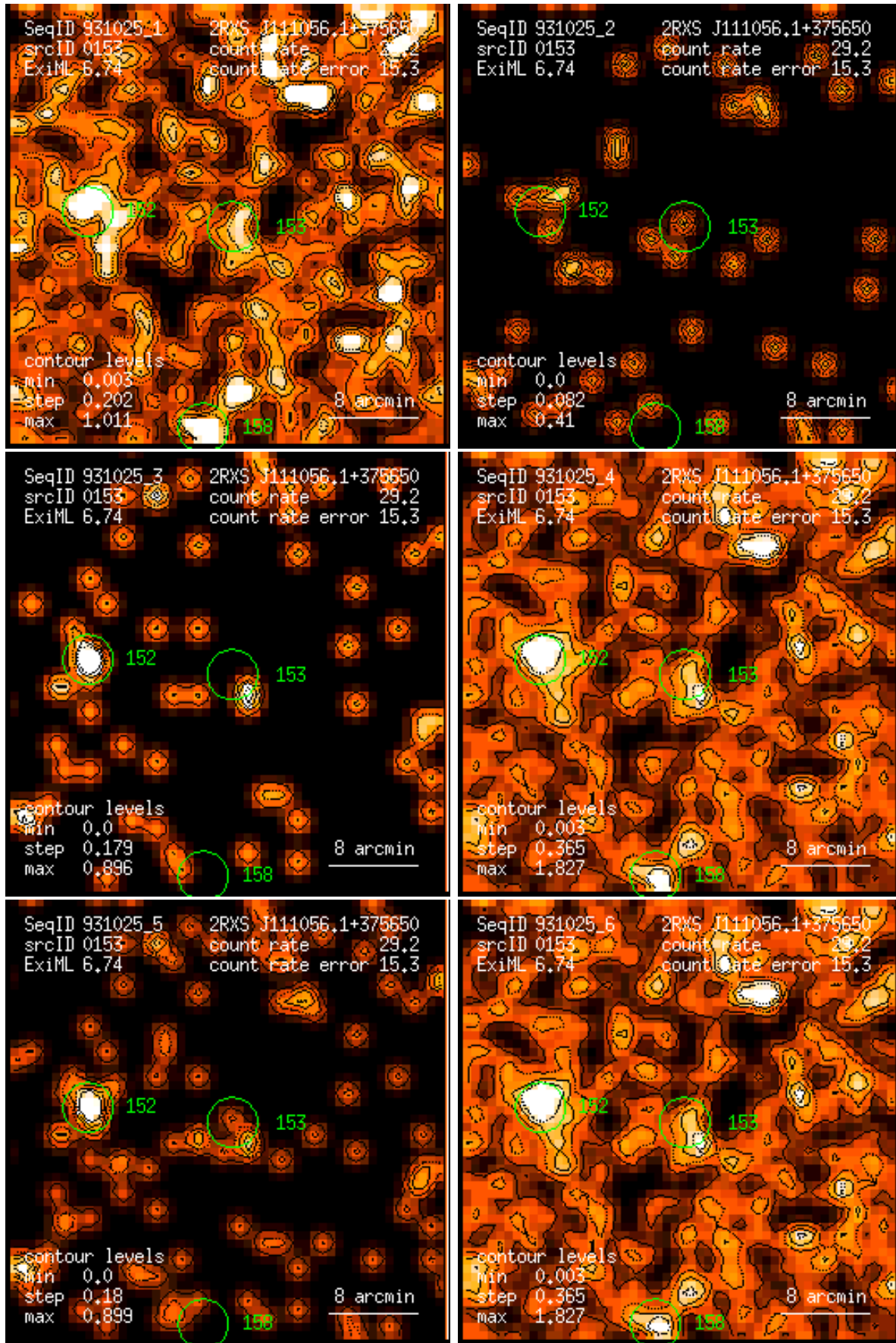
Figure 153: RASS 931025: detection 0153: band rate images, Gaussian filter: (1) PSPC channels 11 – 41, (2) 52 – 90, (3) 91 – 201, (4) 11 – 235, (5) 52 – 201, (6) 11 – 201. Broad band rates in counts/ks. Band rate contour levels in counts/ks/arcmin 2 .
