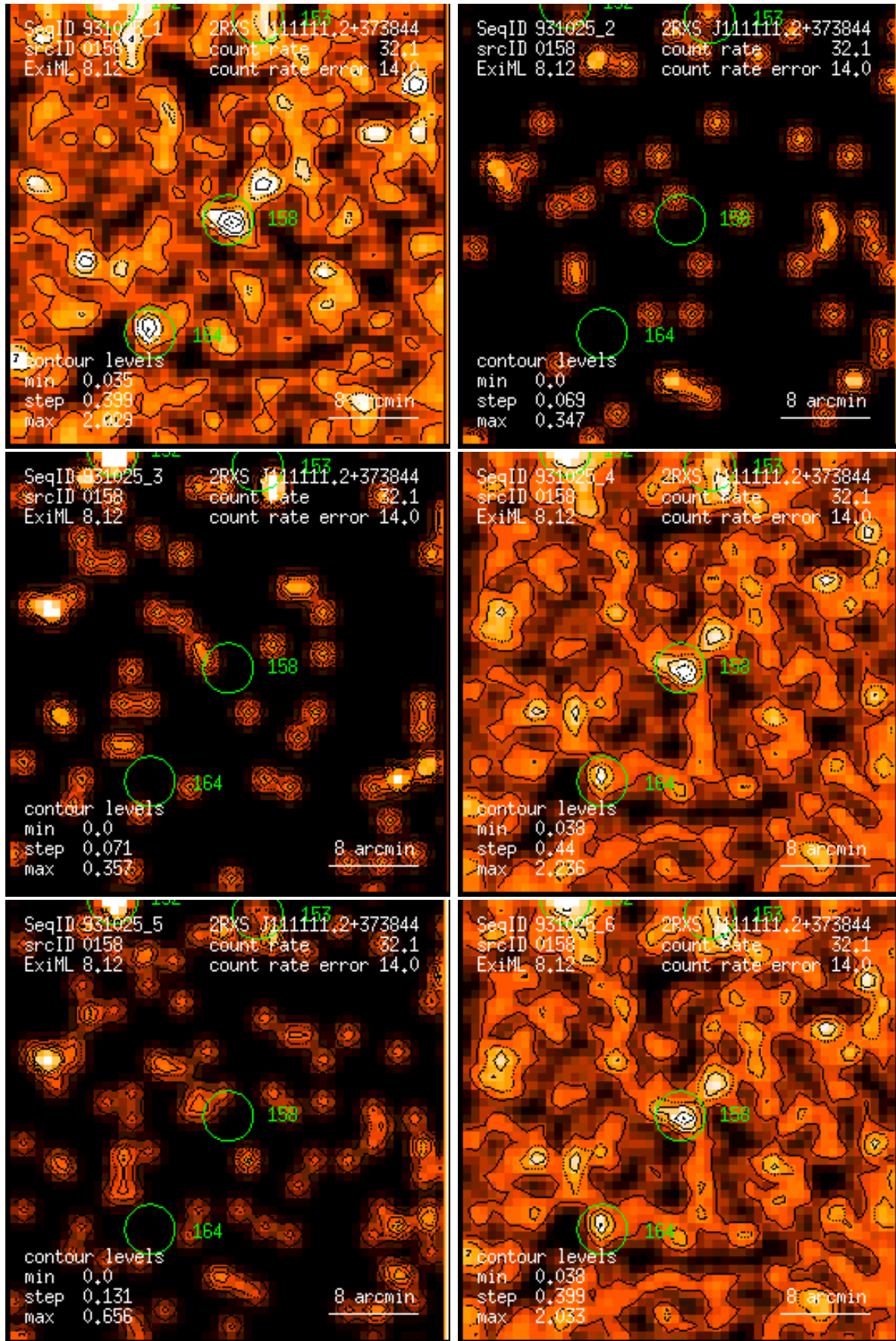
Figure 158: RASS 931025: detection 0158: band rate images, Gaussian filter: (1) PSPC channels 11 – 41, (2) 52 – 90, (3) 91 – 201, (4) 11 – 235, (5) 52 – 201, (6) 11 – 201. Broad band rates in counts/ks. Band rate contour levels in counts/ks/arcmin 2 .
