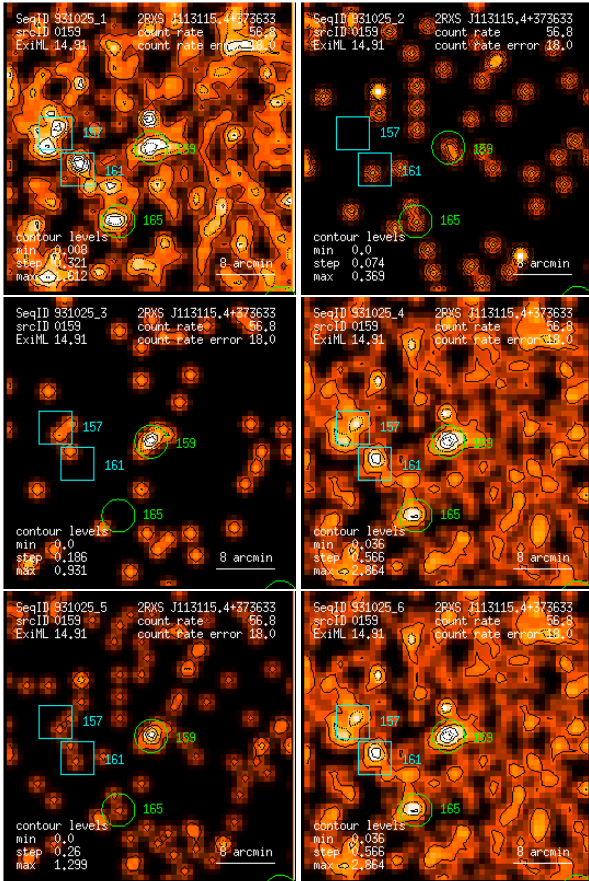
Figure 159: RASS 931025: detection 0159: band rate images, Gaussian filter: (1) PSPC channels 11 – 41, (2) 52 – 90, (3) 91 – 201, (4) 11 – 235, (5) 52 – 201, (6) 11 – 201. Broad band rates in counts/ks. Band rate contour levels in counts/ks/arcmin 2 .
