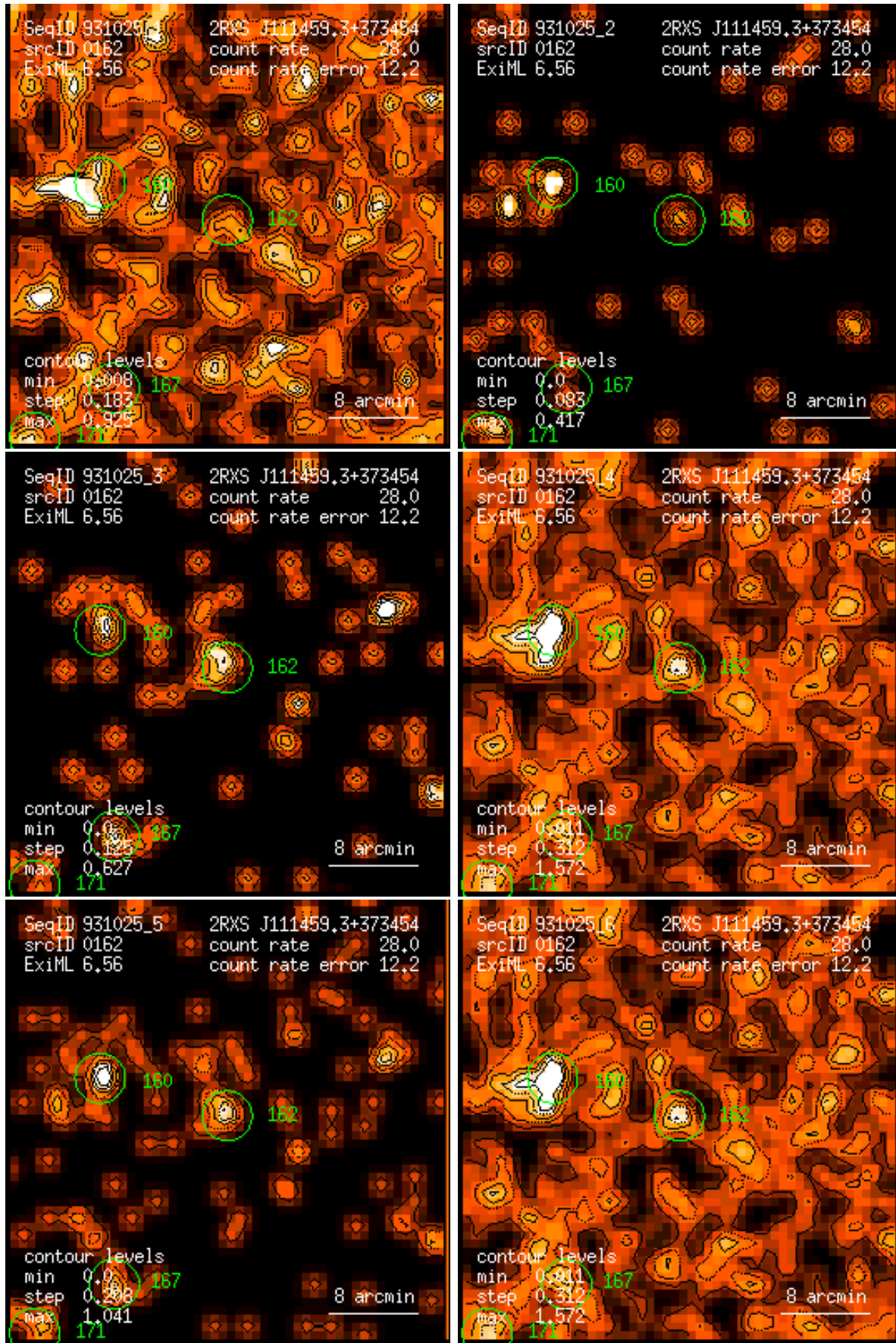
Figure 162: RASS 931025: detection 0162: band rate images, Gaussian filter: (1) PSPC channels 11 – 41, (2) 52 – 90, (3) 91 – 201, (4) 11 – 235, (5) 52 – 201, (6) 11 – 201. Broad band rates in counts/ks. Band rate contour levels in counts/ks/arcmin 2 .
