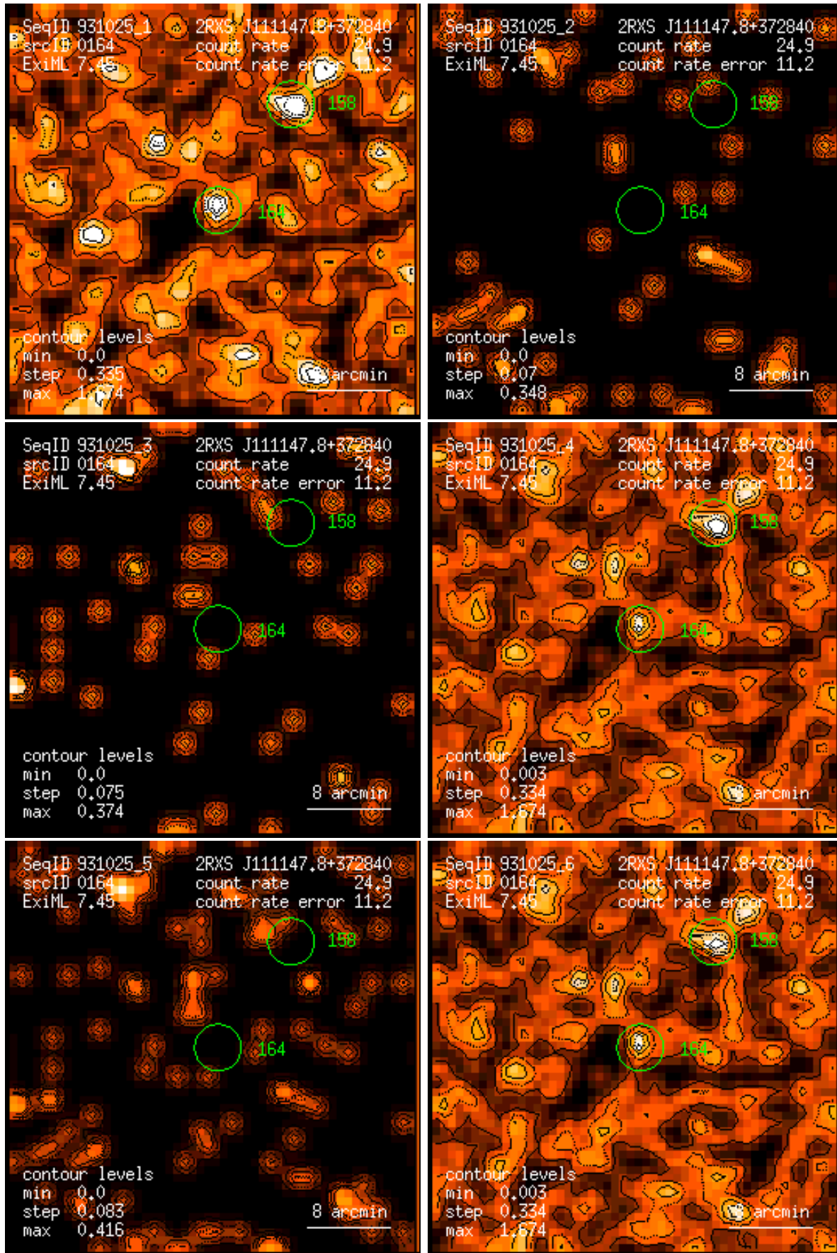
Figure 164: RASS 931025: detection 0164: band rate images, Gaussian filter: (1) PSPC channels 11 – 41, (2) 52 – 90, (3) 91 – 201, (4) 11 – 235, (5) 52 – 201, (6) 11 – 201. Broad band rates in counts/ks. Band rate contour levels in counts/ks/arcmin 2 .
