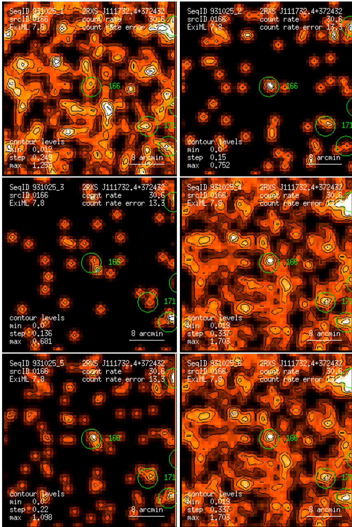
Figure 166: RASS 931025: detection 0166: band rate images, Gaussian filter: (1) PSPC channels 11 – 41, (2) 52 – 90, (3) 91 – 201, (4) 11 – 235, (5) 52 – 201, (6) 11 – 201. Broad band rates in counts/ks. Band rate contour levels in counts/ks/arcmin 2 .
