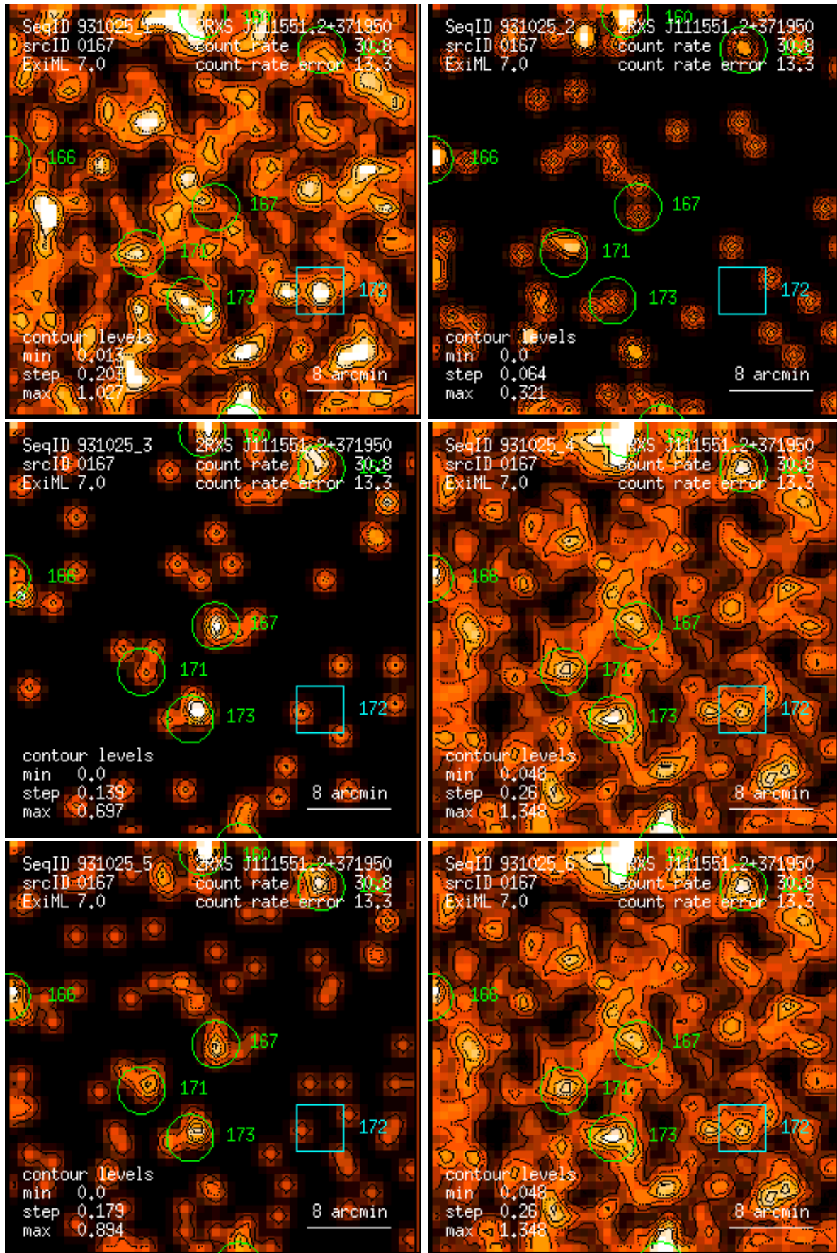
Figure 167: RASS 931025: detection 0167: band rate images, Gaussian filter: (1) PSPC channels 11 – 41, (2) 52 – 90, (3) 91 – 201, (4) 11 – 235, (5) 52 – 201, (6) 11 – 201. Broad band rates in counts/ks. Band rate contour levels in counts/ks/arcmin 2 .
