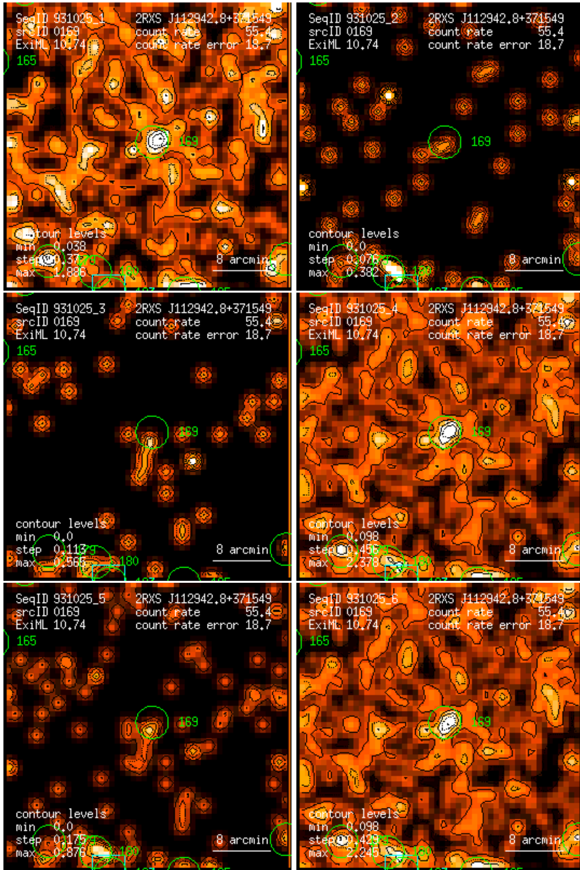
Figure 169: RASS 931025: detection 0169: band rate images, Gaussian filter: (1) PSPC channels 11 – 41, (2) 52 – 90, (3) 91 – 201, (4) 11 – 235, (5) 52 – 201, (6) 11 – 201. Broad band rates in counts/ks. Band rate contour levels in counts/ks/arcmin 2 .
