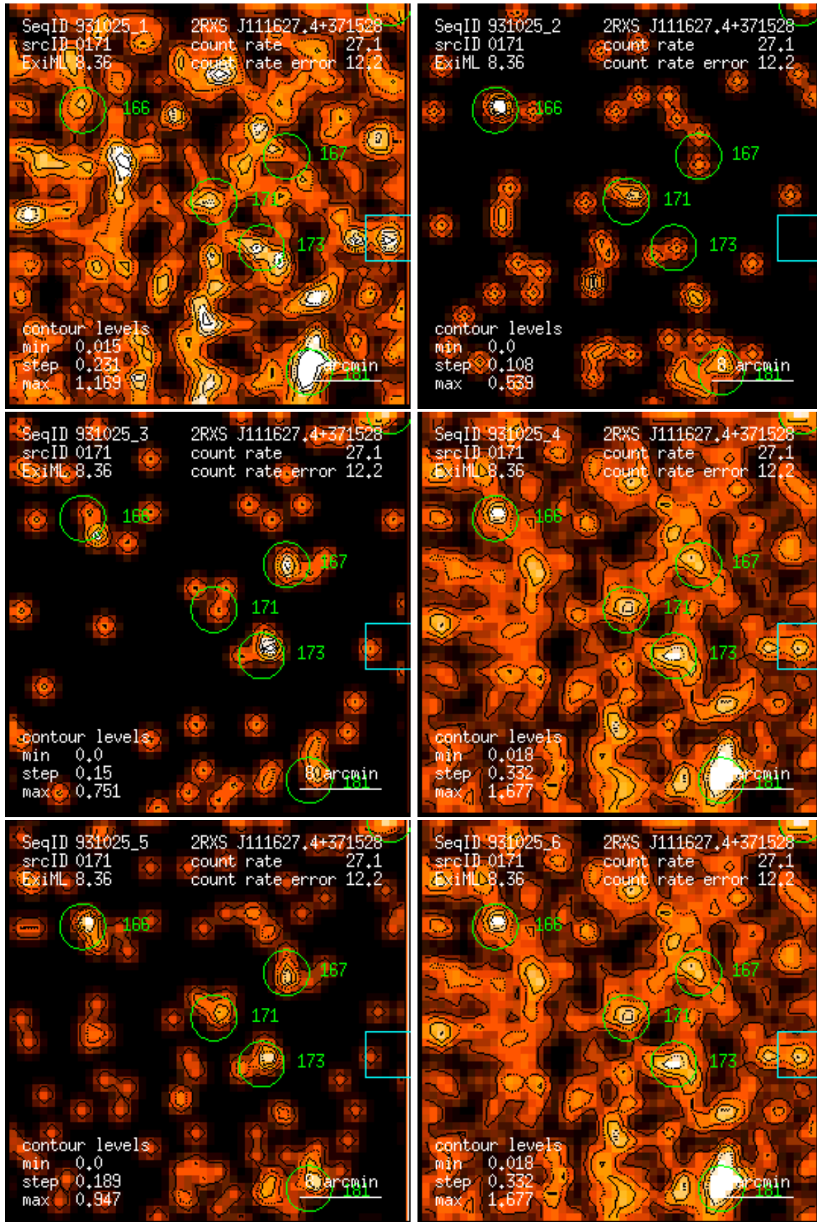
Figure 171: RASS 931025: detection 0171: band rate images, Gaussian filter: (1) PSPC channels 11 – 41, (2) 52 – 90, (3) 91 – 201, (4) 11 – 235, (5) 52 – 201, (6) 11 – 201. Broad band rates in counts/ks. Band rate contour levels in counts/ks/arcmin 2 .
