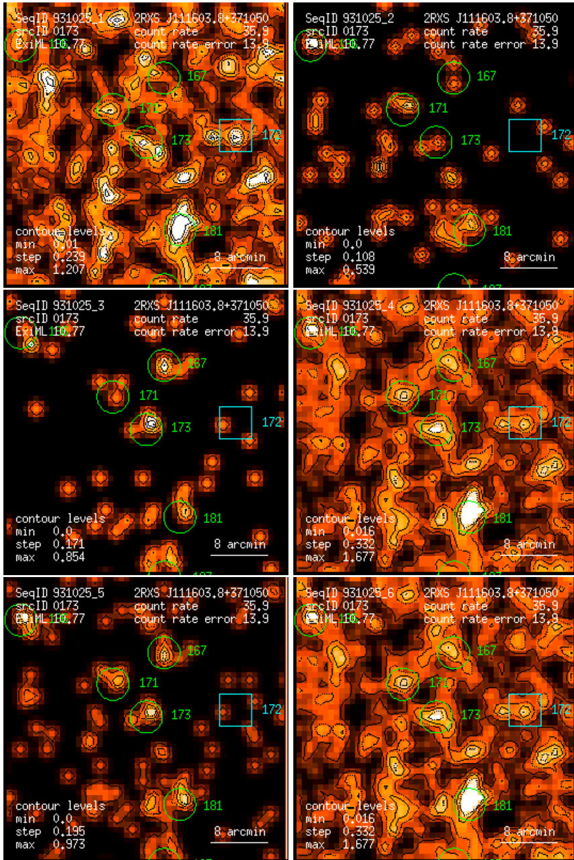
Figure 173: RASS 931025: detection 0173: band rate images, Gaussian filter: (1) PSPC channels 11 – 41, (2) 52 – 90, (3) 91 – 201, (4) 11 – 235, (5) 52 – 201, (6) 11 – 201. Broad band rates in counts/ks. Band rate contour levels in counts/ks/arcmin 2 .
