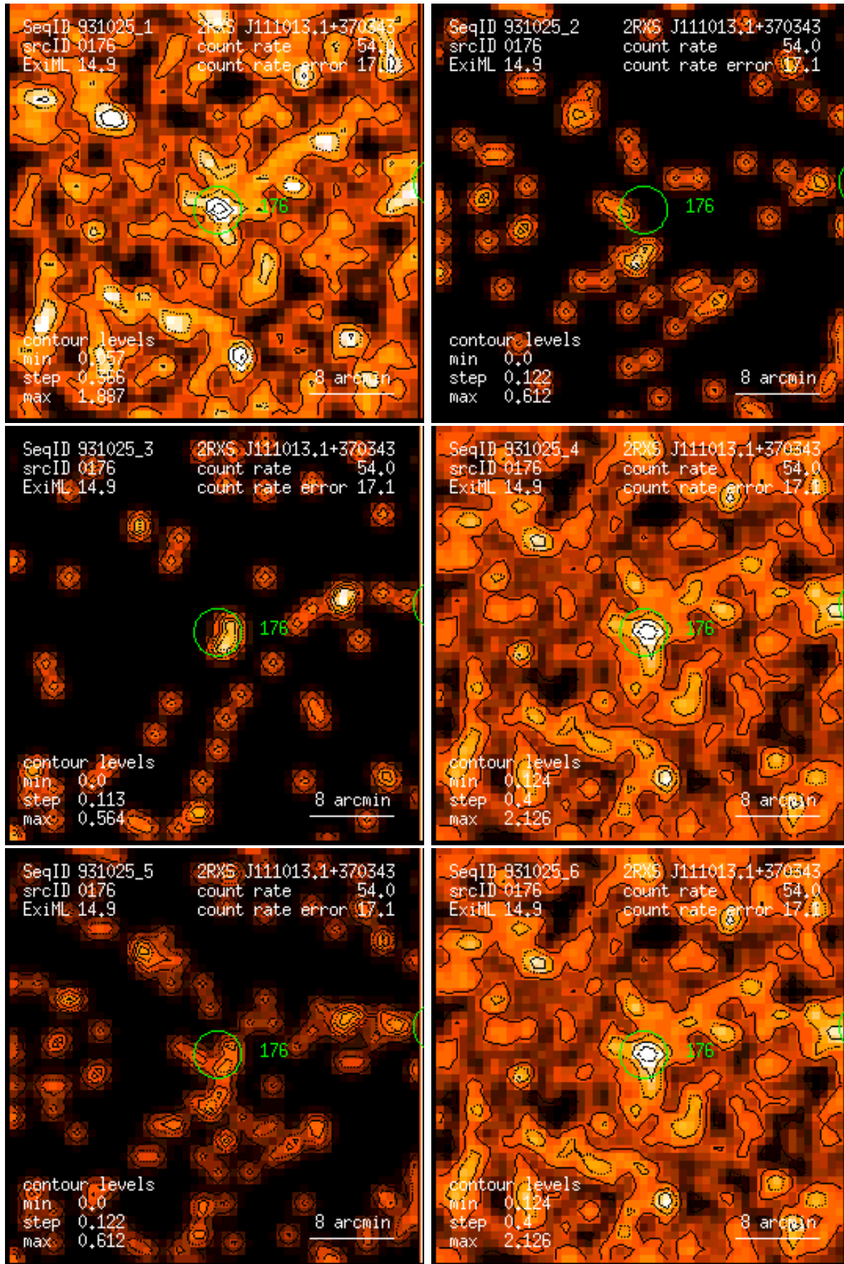
Figure 176: RASS 931025: detection 0176: band rate images, Gaussian filter: (1) PSPC channels 11 – 41, (2) 52 – 90, (3) 91 – 201, (4) 11 – 235, (5) 52 – 201, (6) 11 – 201. Broad band rates in counts/ks. Band rate contour levels in counts/ks/arcmin 2 .
