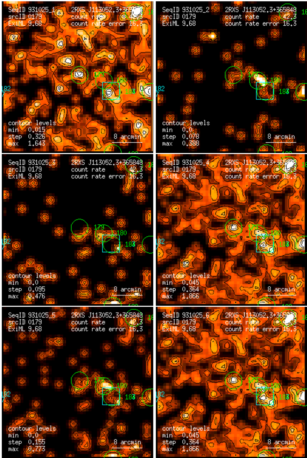
Figure 179: RASS 931025: detection 0179: band rate images, Gaussian filter: (1) PSPC channels 11 – 41, (2) 52 – 90, (3) 91 – 201, (4) 11 – 235, (5) 52 – 201, (6) 11 – 201. Broad band rates in counts/ks. Band rate contour levels in counts/ks/arcmin 2 .
