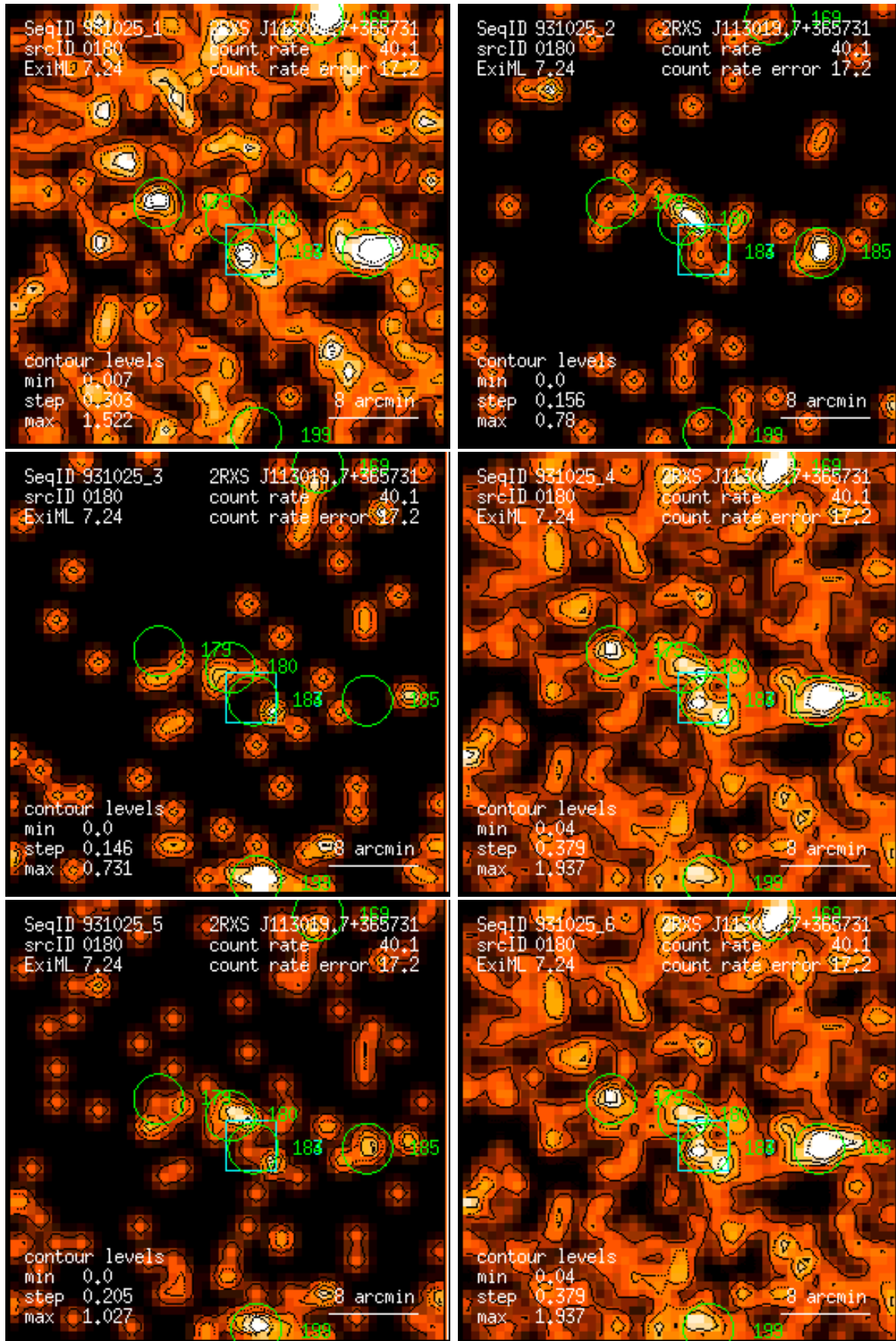
Figure 180: RASS 931025: detection 0180: band rate images, Gaussian filter: (1) PSPC channels 11 – 41, (2) 52 – 90, (3) 91 – 201, (4) 11 – 235, (5) 52 – 201, (6) 11 – 201. Broad band rates in counts/ks. Band rate contour levels in counts/ks/arcmin 2 .
