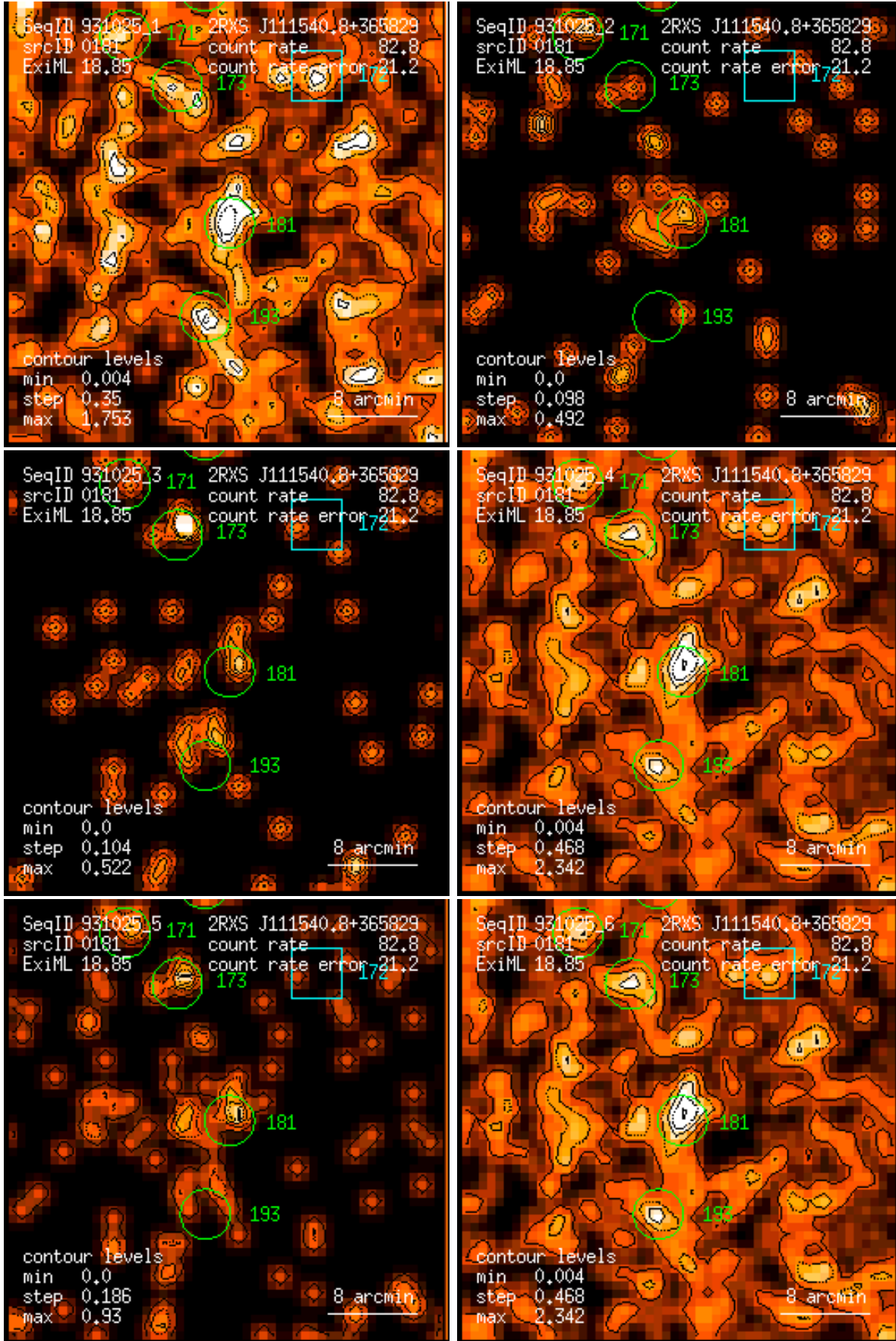
Figure 181: RASS 931025: detection 0181: band rate images, Gaussian filter: (1) PSPC channels 11 – 41, (2) 52 – 90, (3) 91 – 201, (4) 11 – 235, (5) 52 – 201, (6) 11 – 201. Broad band rates in counts/ks. Band rate contour levels in counts/ks/arcmin 2 .
