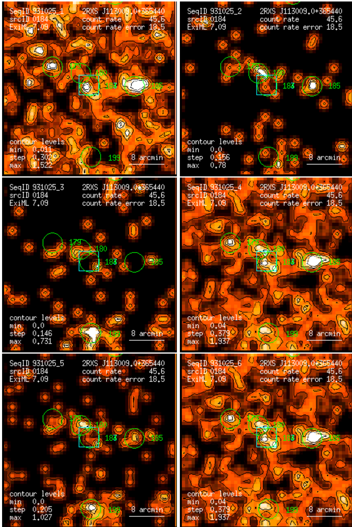
Figure 184: RASS 931025: detection 0184: band rate images, Gaussian filter: (1) PSPC channels 11 – 41, (2) 52 – 90, (3) 91 – 201, (4) 11 – 235, (5) 52 – 201, (6) 11 – 201. Broad band rates in counts/ks. Band rate contour levels in counts/ks/arcmin 2 .
