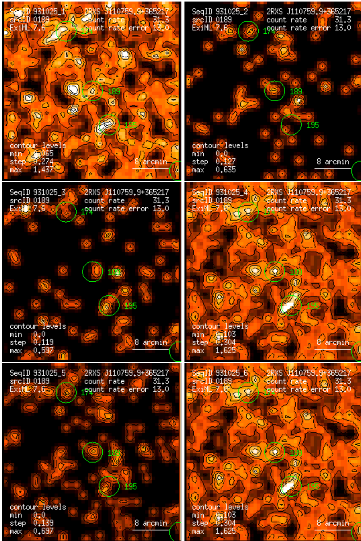
Figure 189: RASS 931025: detection 0189: band rate images, Gaussian filter: (1) PSPC channels 11 – 41, (2) 52 – 90, (3) 91 – 201, (4) 11 – 235, (5) 52 – 201, (6) 11 – 201. Broad band rates in counts/ks. Band rate contour levels in counts/ks/arcmin 2 .
