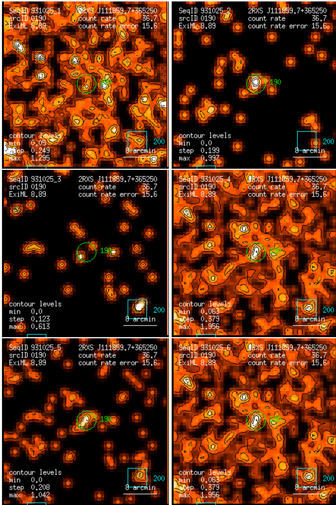
Figure 190: RASS 931025: detection 0190: band rate images, Gaussian filter: (1) PSPC channels 11 – 41, (2) 52 – 90, (3) 91 – 201, (4) 11 – 235, (5) 52 – 201, (6) 11 – 201. Broad band rates in counts/ks. Band rate contour levels in counts/ks/arcmin 2 .
