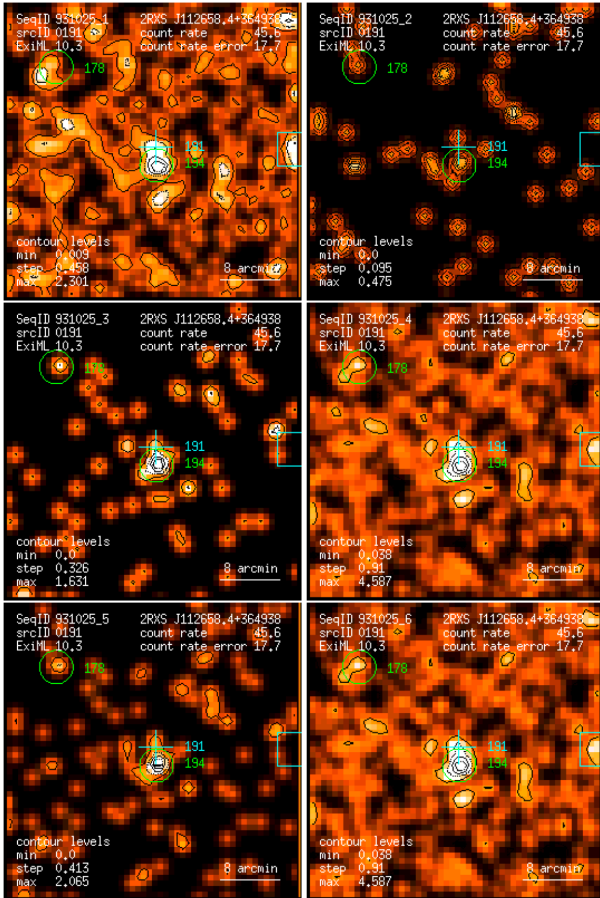
Figure 191: RASS 931025: detection 0191: band rate images, Gaussian filter: (1) PSPC channels 11 – 41, (2) 52 – 90, (3) 91 – 201, (4) 11 – 235, (5) 52 – 201, (6) 11 – 201. Broad band rates in counts/ks. Band rate contour levels in counts/ks/arcmin 2 .
