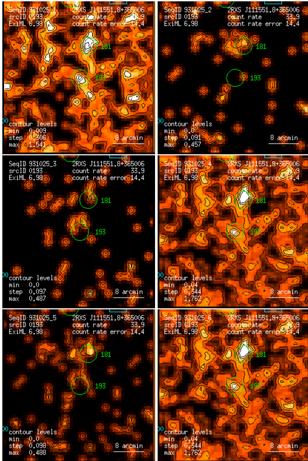
Figure 193: RASS 931025: detection 0193: band rate images, Gaussian filter: (1) PSPC channels 11 – 41, (2) 52 – 90, (3) 91 – 201, (4) 11 – 235, (5) 52 – 201, (6) 11 – 201. Broad band rates in counts/ks. Band rate contour levels in counts/ks/arcmin 2 .
