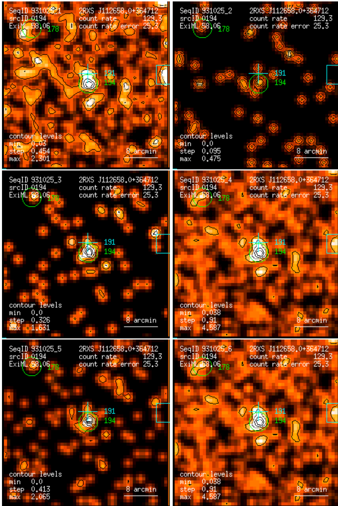
Figure 194: RASS 931025: detection 0194: band rate images, Gaussian filter: (1) PSPC channels 11 – 41, (2) 52 – 90, (3) 91 – 201, (4) 11 – 235, (5) 52 – 201, (6) 11 – 201. Broad band rates in counts/ks. Band rate contour levels in counts/ks/arcmin 2 .
