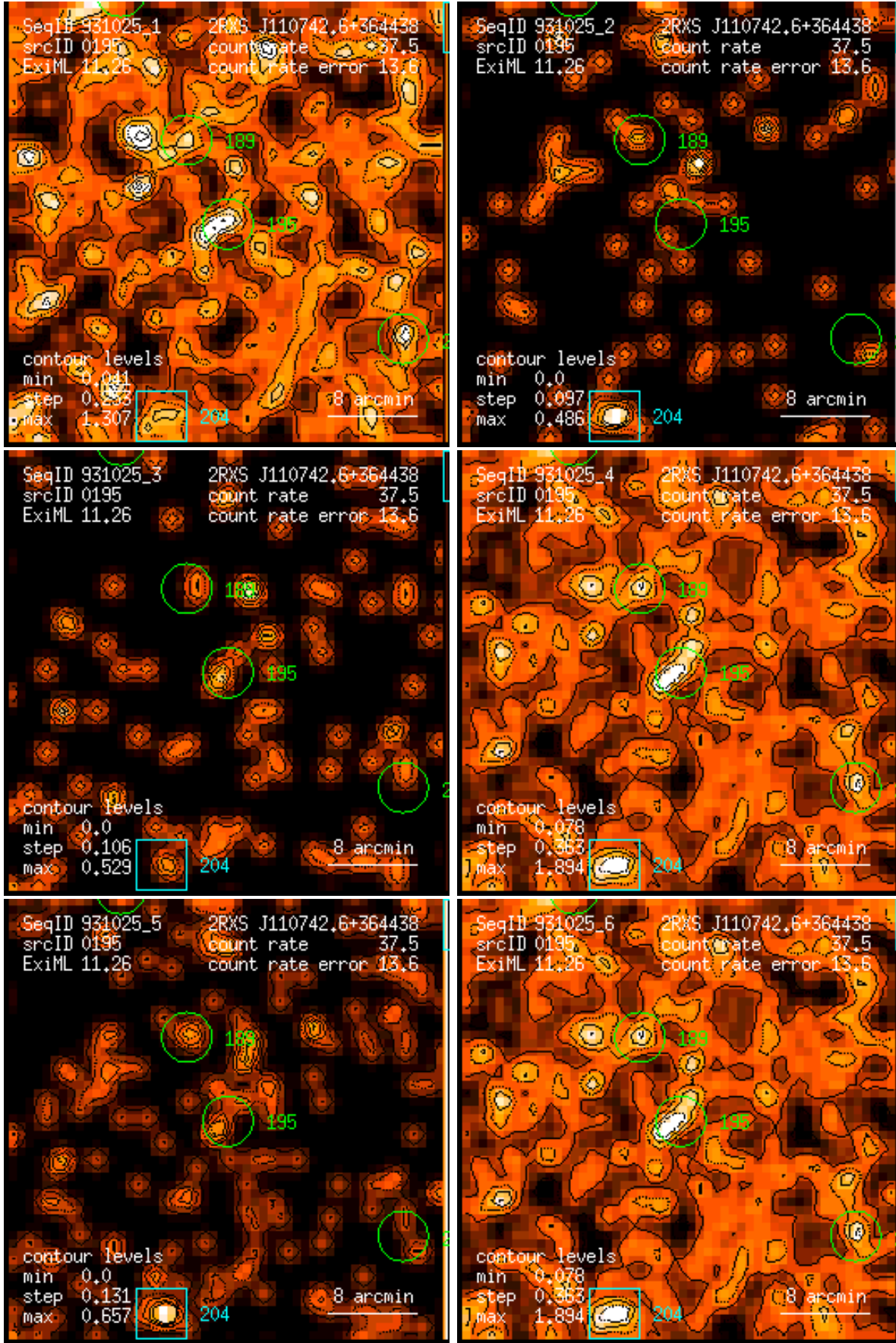
Figure 195: RASS 931025: detection 0195: band rate images, Gaussian filter: (1) PSPC channels 11 – 41, (2) 52 – 90, (3) 91 – 201, (4) 11 – 235, (5) 52 – 201, (6) 11 – 201. Broad band rates in counts/ks. Band rate contour levels in counts/ks/arcmin 2 .
