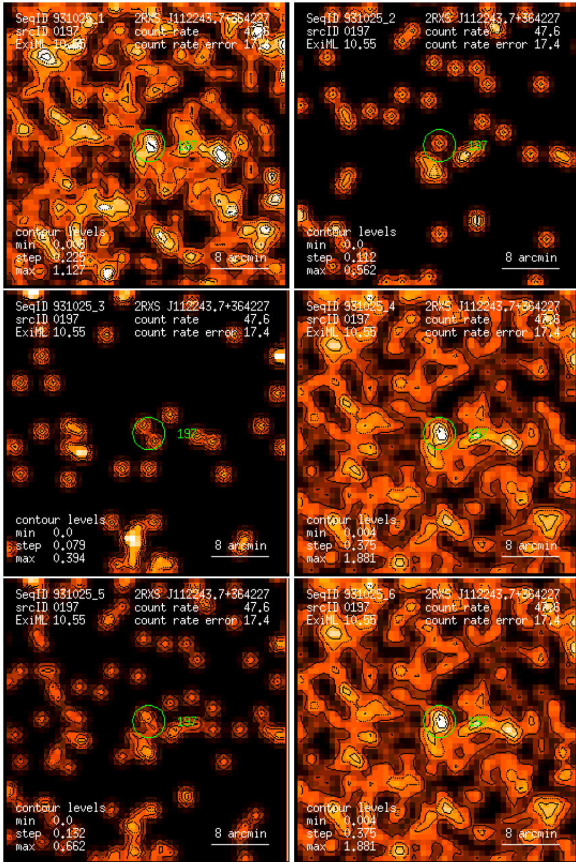
Figure 197: RASS 931025: detection 0197: band rate images, Gaussian filter: (1) PSPC channels 11 – 41, (2) 52 – 90, (3) 91 – 201, (4) 11 – 235, (5) 52 – 201, (6) 11 – 201. Broad band rates in counts/ks. Band rate contour levels in counts/ks/arcmin 2 .
