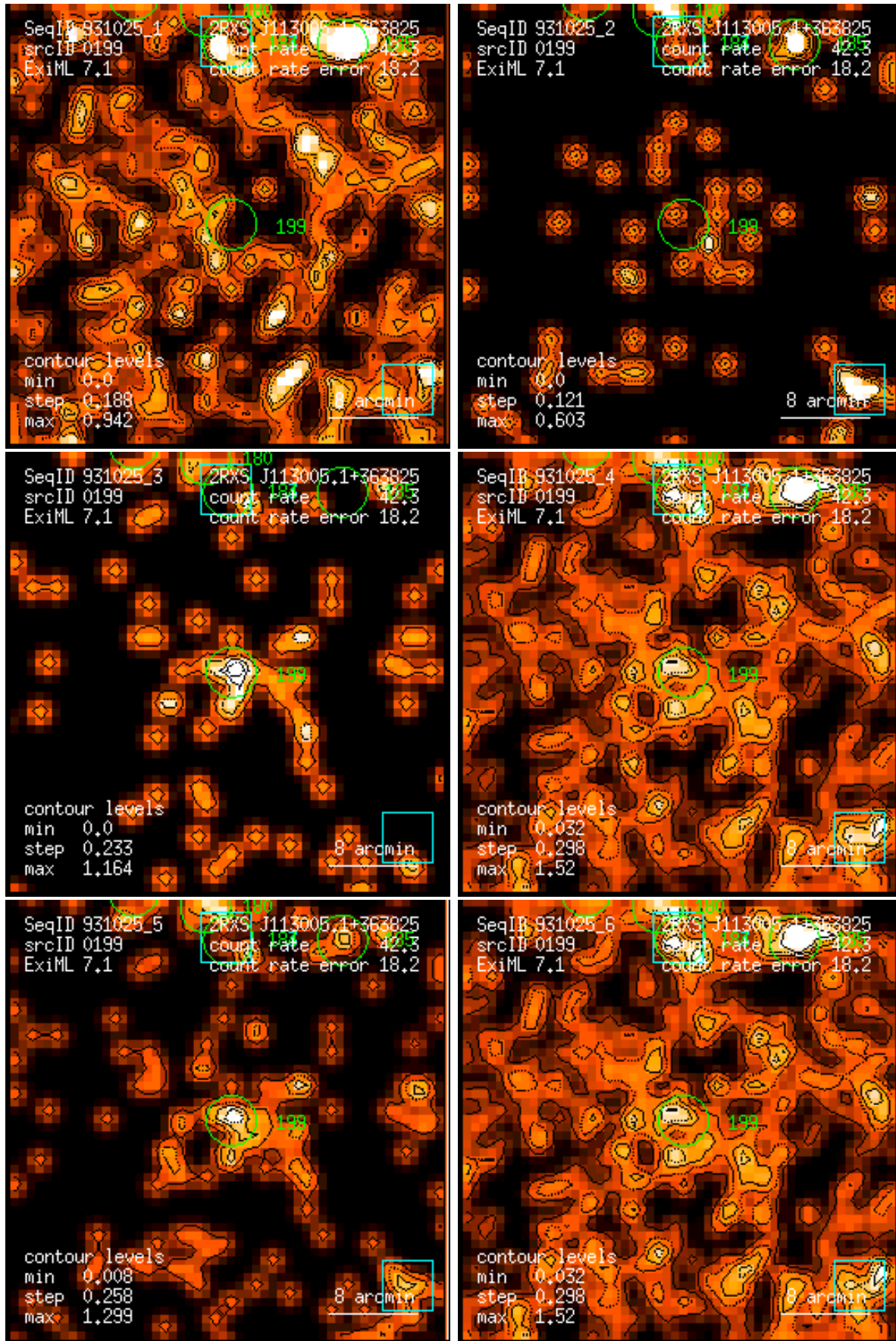
Figure 199: RASS 931025: detection 0199: band rate images, Gaussian filter: (1) PSPC channels 11 – 41, (2) 52 – 90, (3) 91 – 201, (4) 11 – 235, (5) 52 – 201, (6) 11 – 201. Broad band rates in counts/ks. Band rate contour levels in counts/ks/arcmin 2 .
