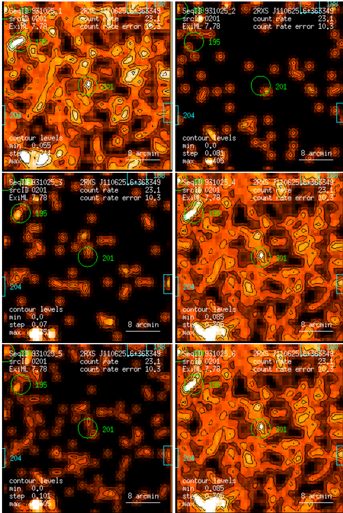
Figure 201: RASS 931025: detection 0201: band rate images, Gaussian filter: (1) PSPC channels 11 – 41, (2) 52 – 90, (3) 91 – 201, (4) 11 – 235, (5) 52 – 201, (6) 11 – 201. Broad band rates in counts/ks. Band rate contour levels in counts/ks/arcmin 2 .
