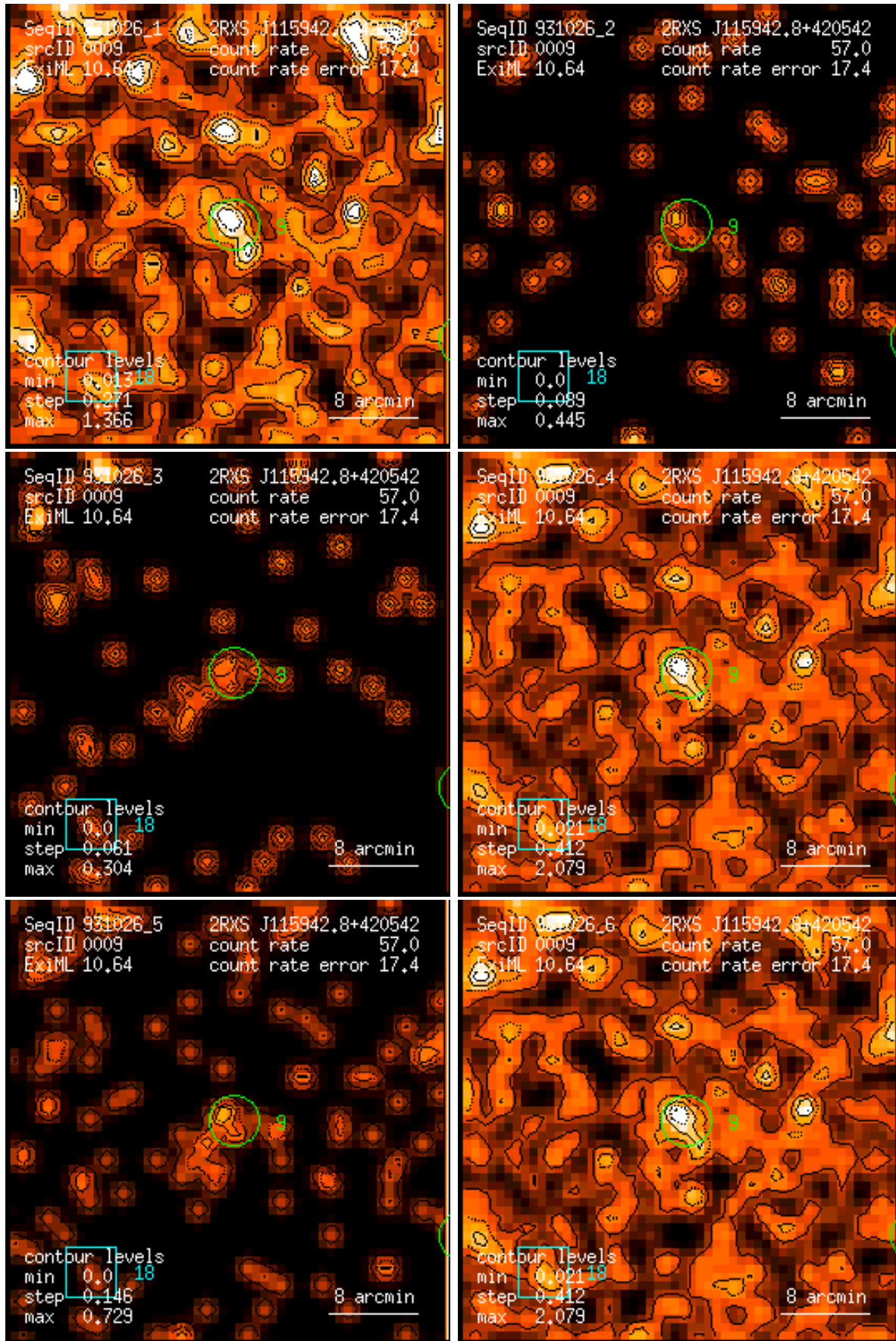
Figure 9: RASS 931026: detection 0009: band rate images, Gaussian filter: (1) PSPC channels 11 – 41, (2) 52 – 90, (3) 91 – 201, (4) 11 – 235, (5) 52 – 201, (6) 11 – 201. Broad band rates in counts/ks. Band rate contour levels in counts/ks/arcmin 2 .
