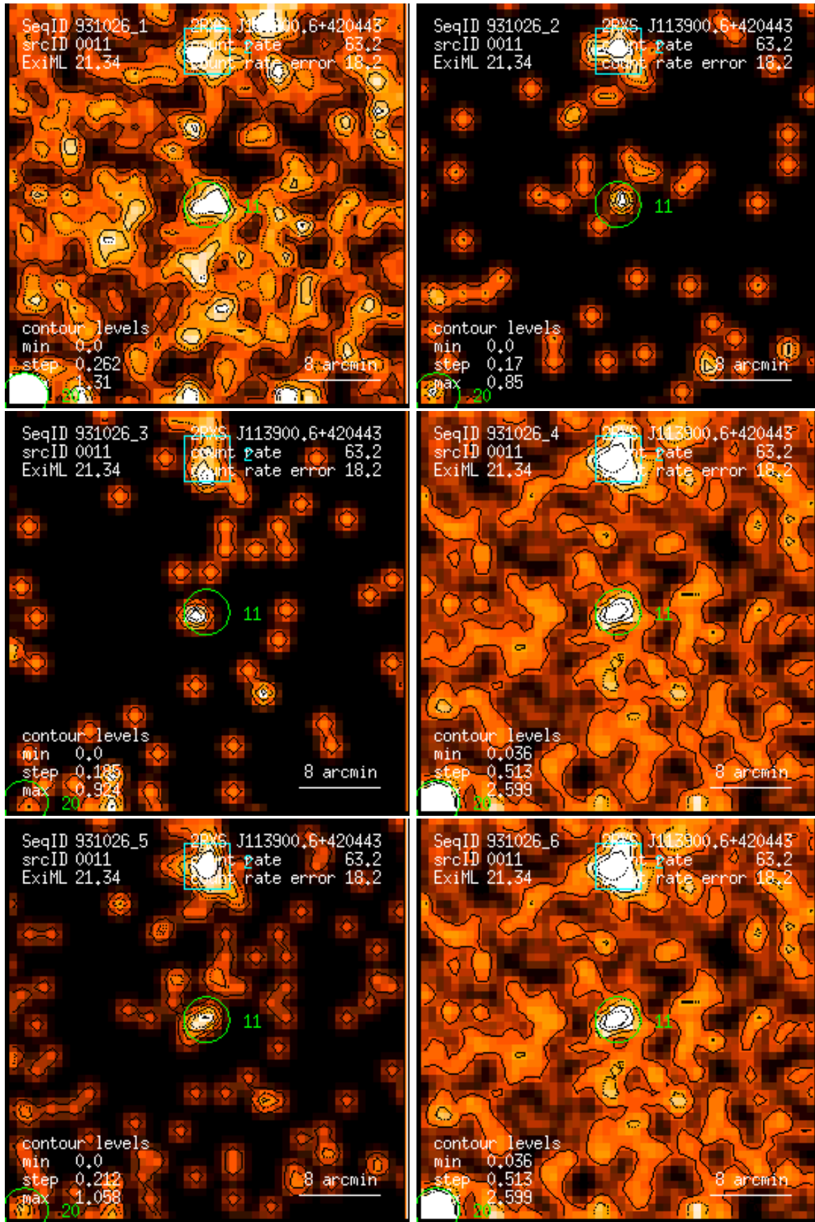
Figure 11: RASS 931026: detection 0011: band rate images, Gaussian filter: (1) PSPC channels 11 – 41, (2) 52 – 90, (3) 91 – 201, (4) 11 – 235, (5) 52 – 201, (6) 11 – 201. Broad band rates in counts/ks. Band rate contour levels in counts/ks/arcmin 2 .
