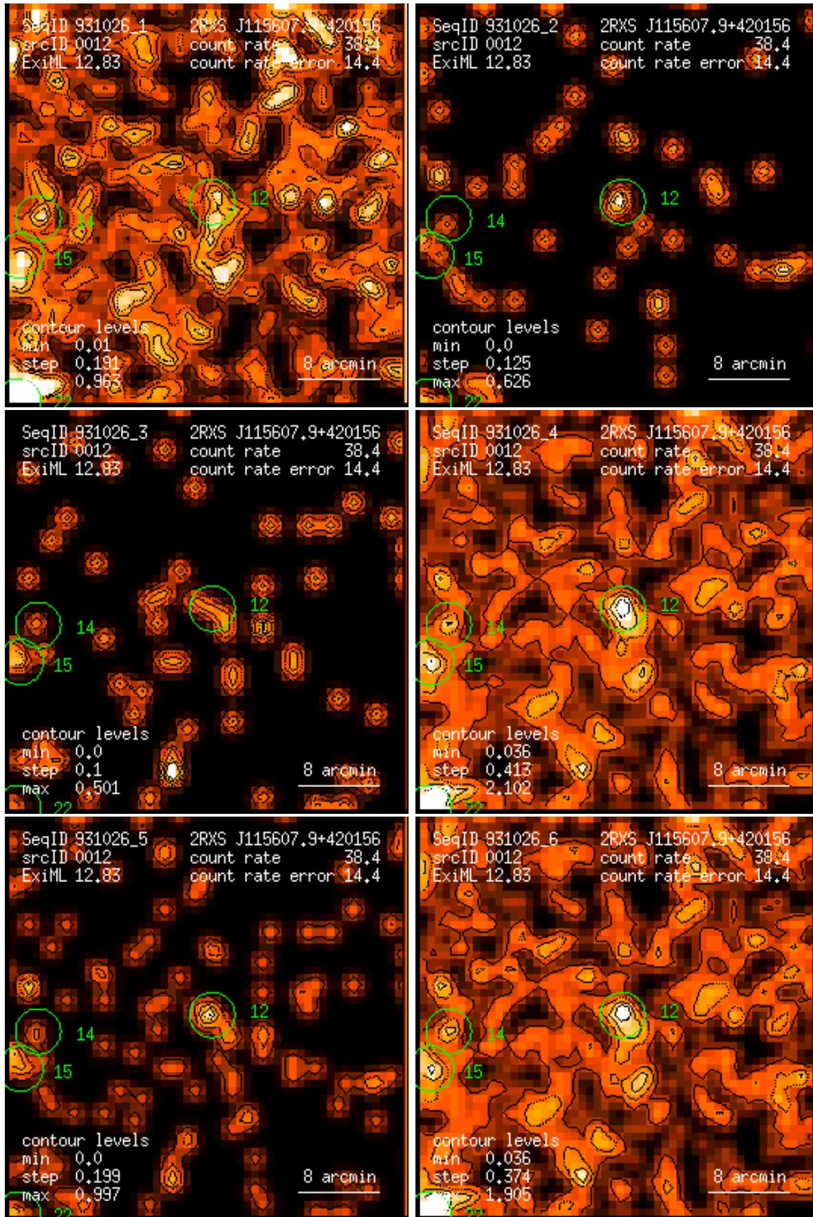
Figure 12: RASS 931026: detection 0012: band rate images, Gaussian filter: (1) PSPC channels 11 – 41, (2) 52 – 90, (3) 91 – 201, (4) 11 – 235, (5) 52 – 201, (6) 11 – 201. Broad band rates in counts/ks. Band rate contour levels in counts/ks/arcmin 2 .
