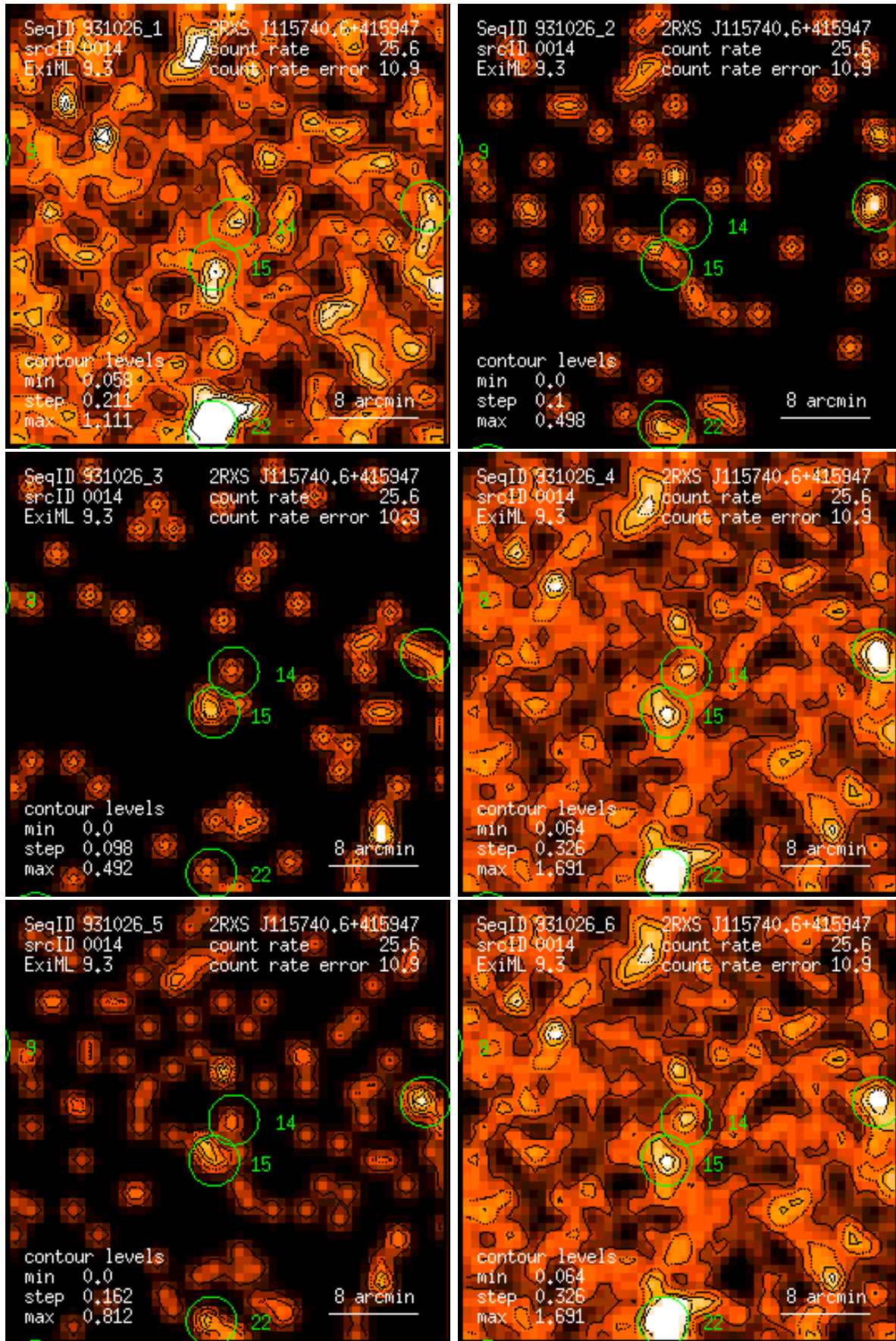
Figure 14: RASS 931026: detection 0014: band rate images, Gaussian filter: (1) PSPC channels 11 – 41, (2) 52 – 90, (3) 91 – 201, (4) 11 – 235, (5) 52 – 201, (6) 11 – 201. Broad band rates in counts/ks. Band rate contour levels in counts/ks/arcmin 2 .
