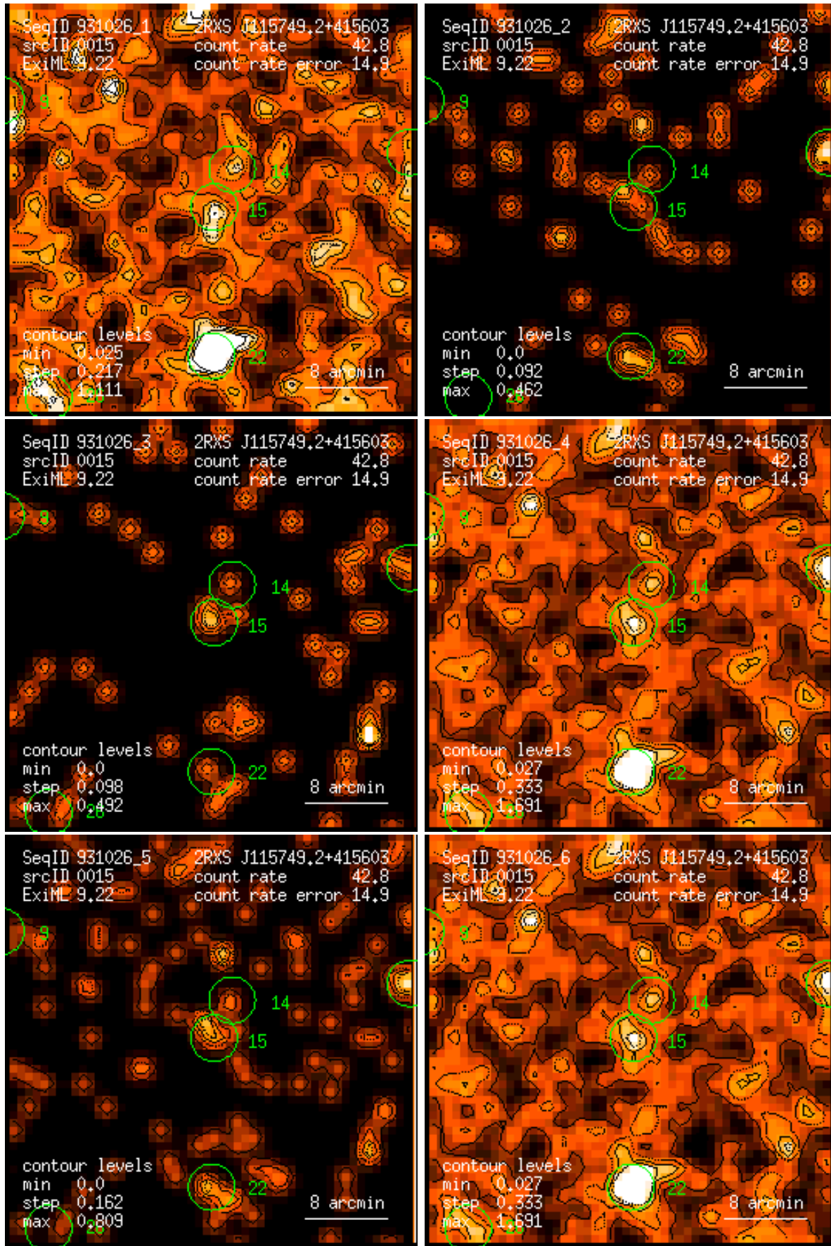
Figure 15: RASS 931026: detection 0015: band rate images, Gaussian filter: (1) PSPC channels 11 – 41, (2) 52 – 90, (3) 91 – 201, (4) 11 – 235, (5) 52 – 201, (6) 11 – 201. Broad band rates in counts/ks. Band rate contour levels in counts/ks/arcmin 2 .
