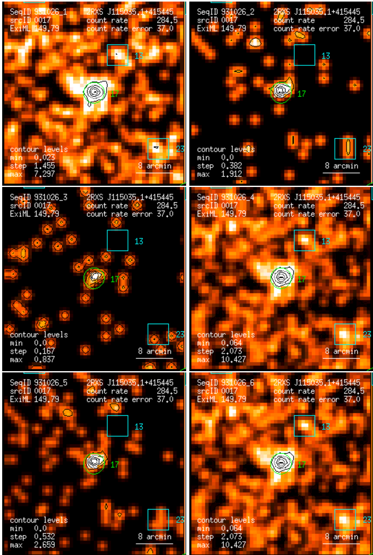
Figure 17: RASS 931026: detection 0017: band rate images, Gaussian filter: (1) PSPC channels 11 – 41, (2) 52 – 90, (3) 91 – 201, (4) 11 – 235, (5) 52 – 201, (6) 11 – 201. Broad band rates in counts/ks. Band rate contour levels in counts/ks/arcmin 2 .
