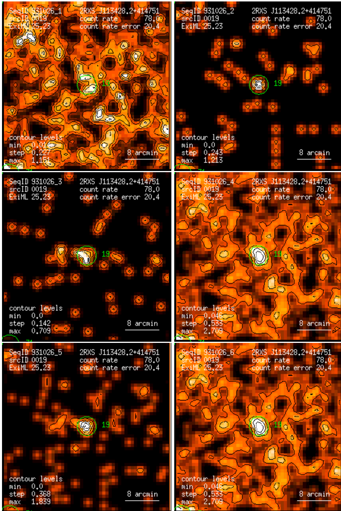
Figure 19: RASS 931026: detection 0019: band rate images, Gaussian filter: (1) PSPC channels 11 – 41, (2) 52 – 90, (3) 91 – 201, (4) 11 – 235, (5) 52 – 201, (6) 11 – 201. Broad band rates in counts/ks. Band rate contour levels in counts/ks/arcmin 2 .
