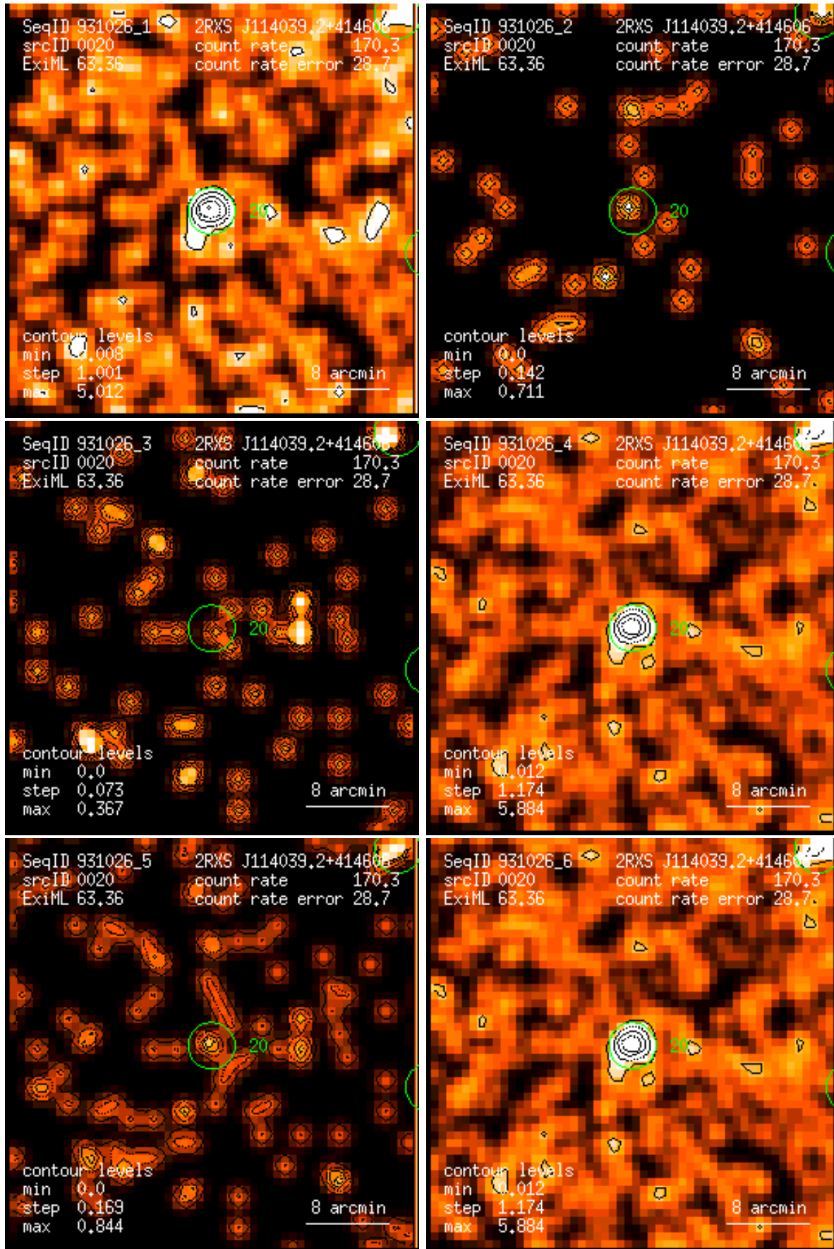
Figure 20: RASS 931026: detection 0020: band rate images, Gaussian filter: (1) PSPC channels 11 – 41, (2) 52 – 90, (3) 91 – 201, (4) 11 – 235, (5) 52 – 201, (6) 11 – 201. Broad band rates in counts/ks. Band rate contour levels in counts/ks/arcmin 2 .
