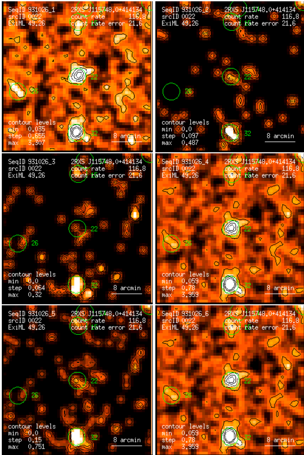
Figure 22: RASS 931026: detection 0022: band rate images, Gaussian filter: (1) PSPC channels 11 – 41, (2) 52 – 90, (3) 91 – 201, (4) 11 – 235, (5) 52 – 201, (6) 11 – 201. Broad band rates in counts/ks. Band rate contour levels in counts/ks/arcmin 2 .
