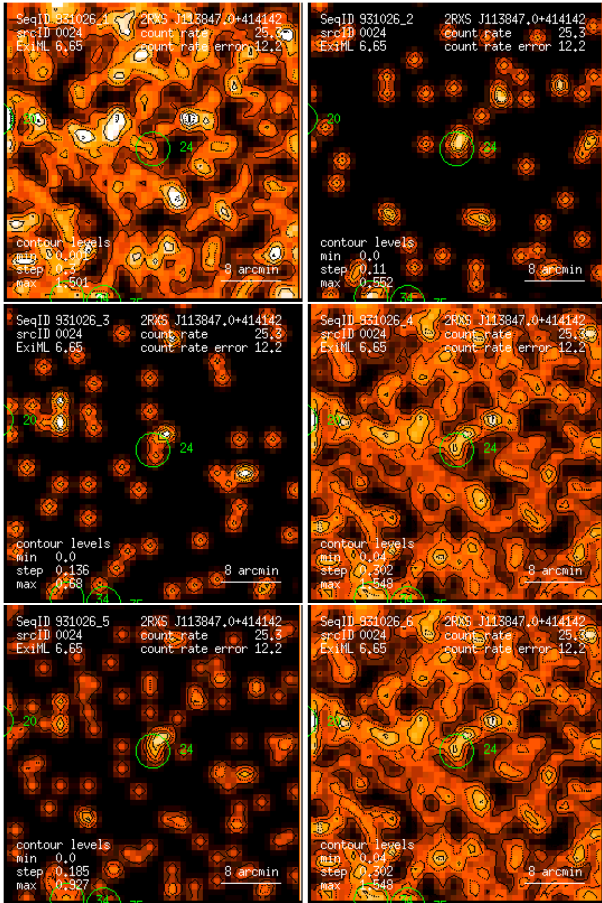
Figure 24: RASS 931026: detection 0024: band rate images, Gaussian filter: (1) PSPC channels 11 – 41, (2) 52 – 90, (3) 91 – 201, (4) 11 – 235, (5) 52 – 201, (6) 11 – 201. Broad band rates in counts/ks. Band rate contour levels in counts/ks/arcmin 2 .
