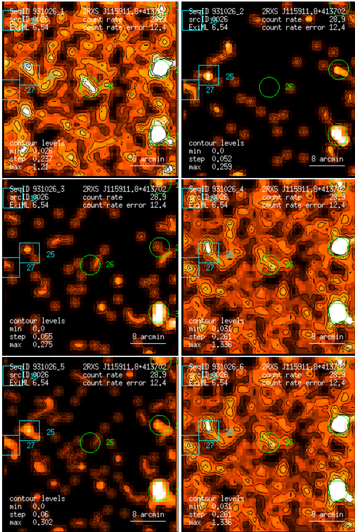
Figure 26: RASS 931026: detection 0026: band rate images, Gaussian filter: (1) PSPC channels 11 – 41, (2) 52 – 90, (3) 91 – 201, (4) 11 – 235, (5) 52 – 201, (6) 11 – 201. Broad band rates in counts/ks. Band rate contour levels in counts/ks/arcmin 2 .
