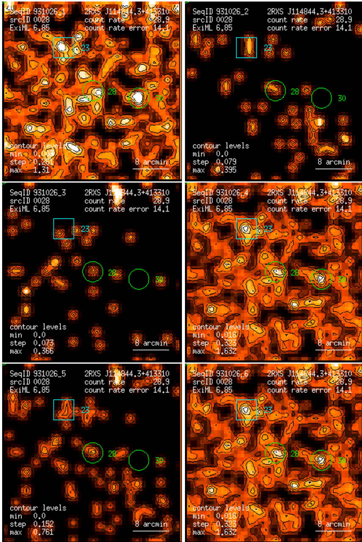
Figure 28: RASS 931026: detection 0028: band rate images, Gaussian filter: (1) PSPC channels 11 – 41, (2) 52 – 90, (3) 91 – 201, (4) 11 – 235, (5) 52 – 201, (6) 11 – 201. Broad band rates in counts/ks. Band rate contour levels in counts/ks/arcmin 2 .
