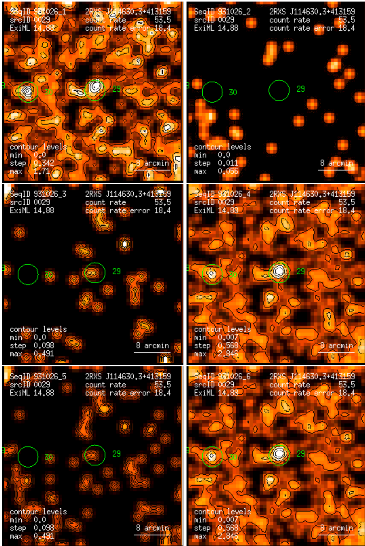
Figure 29: RASS 931026: detection 0029: band rate images, Gaussian filter: (1) PSPC channels 11 – 41, (2) 52 – 90, (3) 91 – 201, (4) 11 – 235, (5) 52 – 201, (6) 11 – 201. Broad band rates in counts/ks. Band rate contour levels in counts/ks/arcmin 2 .
