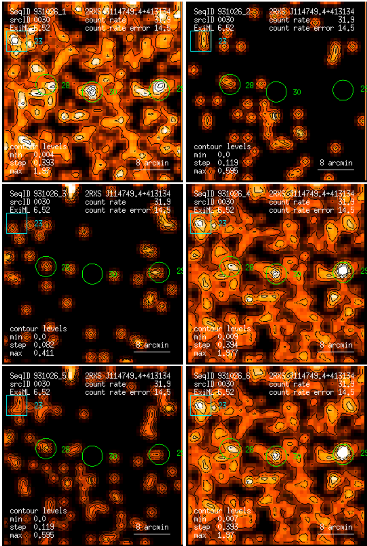
Figure 30: RASS 931026: detection 0030: band rate images, Gaussian filter: (1) PSPC channels 11 – 41, (2) 52 – 90, (3) 91 – 201, (4) 11 – 235, (5) 52 – 201, (6) 11 – 201. Broad band rates in counts/ks. Band rate contour levels in counts/ks/arcmin 2 .
