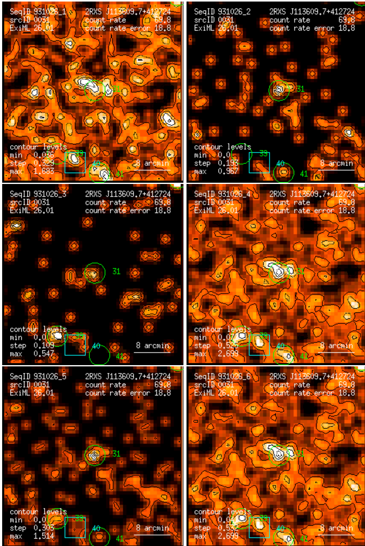
Figure 31: RASS 931026: detection 0031: band rate images, Gaussian filter: (1) PSPC channels 11 – 41, (2) 52 – 90, (3) 91 – 201, (4) 11 – 235, (5) 52 – 201, (6) 11 – 201. Broad band rates in counts/ks. Band rate contour levels in counts/ks/arcmin 2 .
