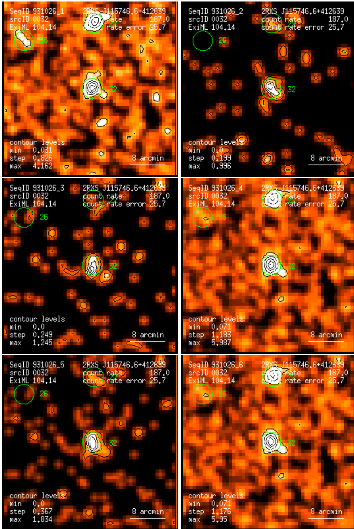
Figure 32: RASS 931026: detection 0032: band rate images, Gaussian filter: (1) PSPC channels 11 – 41, (2) 52 – 90, (3) 91 – 201, (4) 11 – 235, (5) 52 – 201, (6) 11 – 201. Broad band rates in counts/ks. Band rate contour levels in counts/ks/arcmin 2 .
