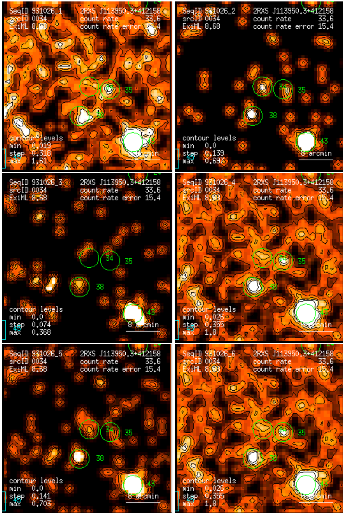
Figure 34: RASS 931026: detection 0034: band rate images, Gaussian filter: (1) PSPC channels 11 – 41, (2) 52 – 90, (3) 91 – 201, (4) 11 – 235, (5) 52 – 201, (6) 11 – 201. Broad band rates in counts/ks. Band rate contour levels in counts/ks/arcmin 2 .
